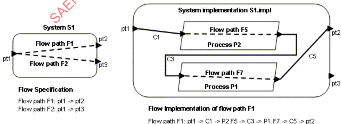
Figure 20 Flow Specification & Flow Implementation
