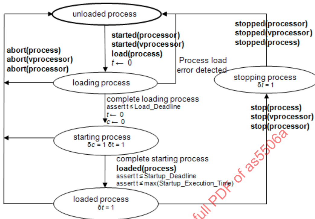
Figure 8 Process States and Actions
