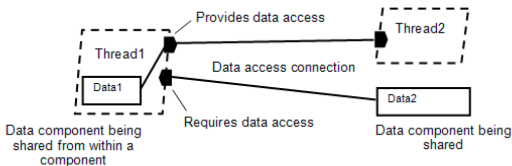
Figure 12 Containment Hierarchy and Shared Access
