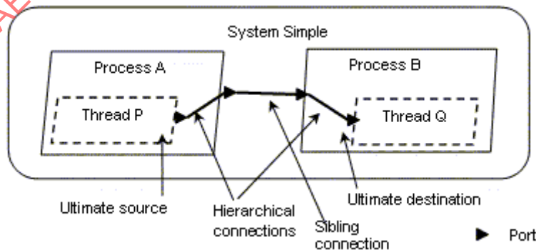
Figure 14 Semantic Port Connection
