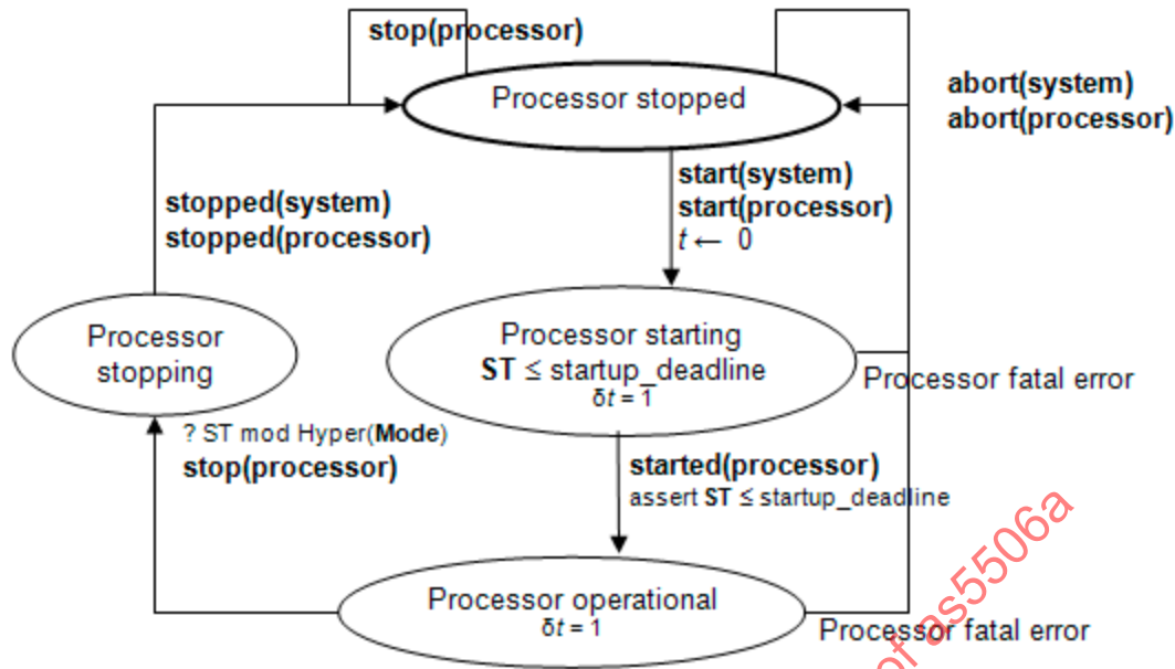
Figure 9 Processor States and Actions
