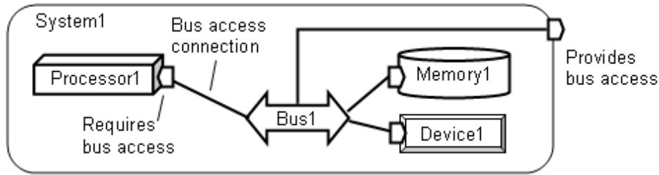
Figure 13 Shared Bus Access
