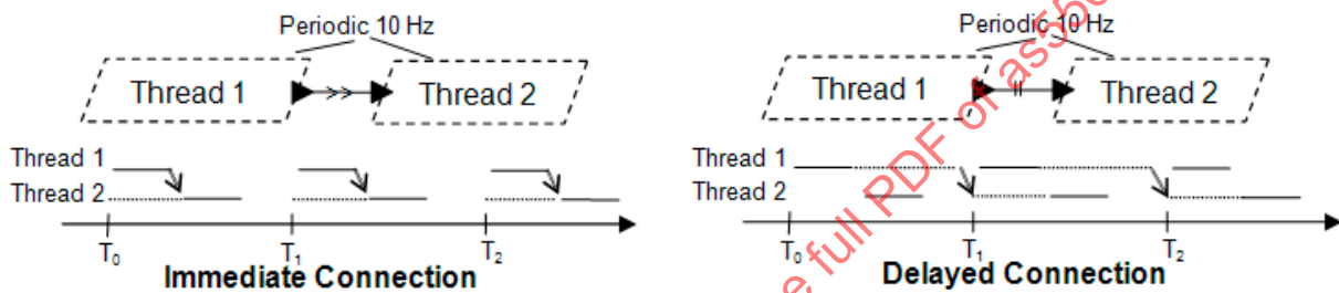
Figure 17 Timing of Immediate & Delayed Data Connections
