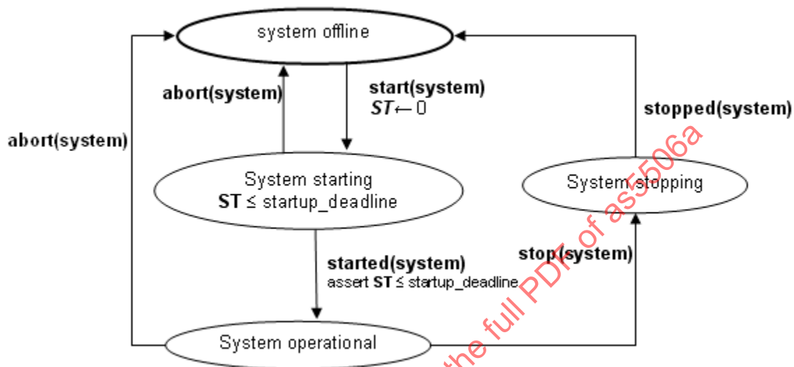
Figure 22 System Instance States, Transitions, and Actions
