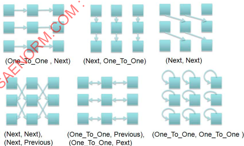
Figure 15 Connection Patterns in 2-Dimensional Component Array
