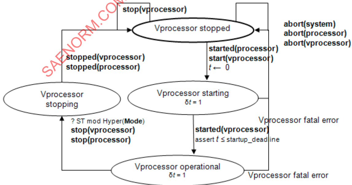
Figure 10 Virtual Processor States and Actions
