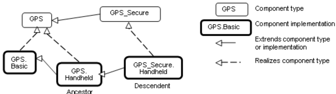
Figure 3 Extension Hierarchy of Component Types and Implementations
