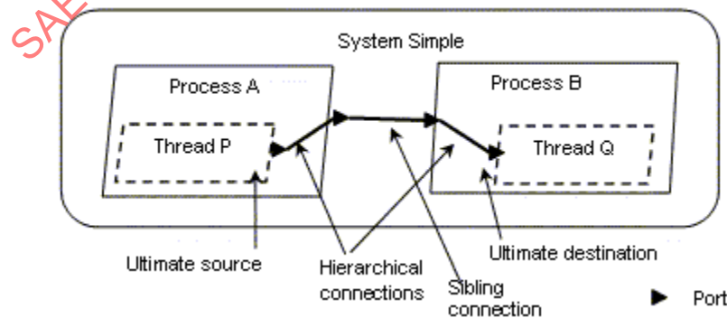
Figure 14 Semantic Port Connection
