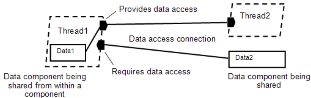
Figure 12 Containment Hierarchy and Shared Access
