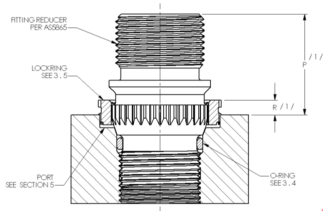
FIGURE 2 - Installed Fitting Reducer Assembly
