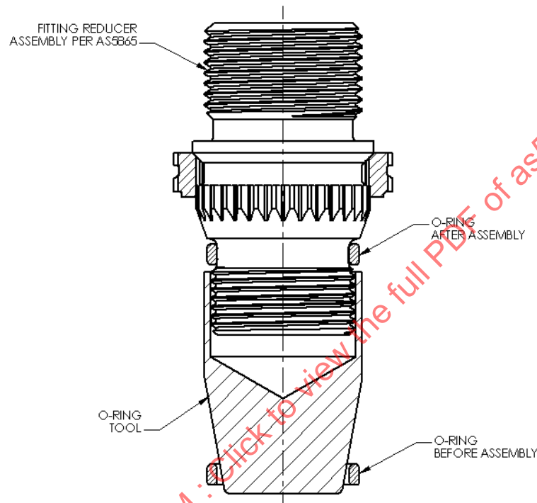
FIGURE 7 - O-ring Installation
