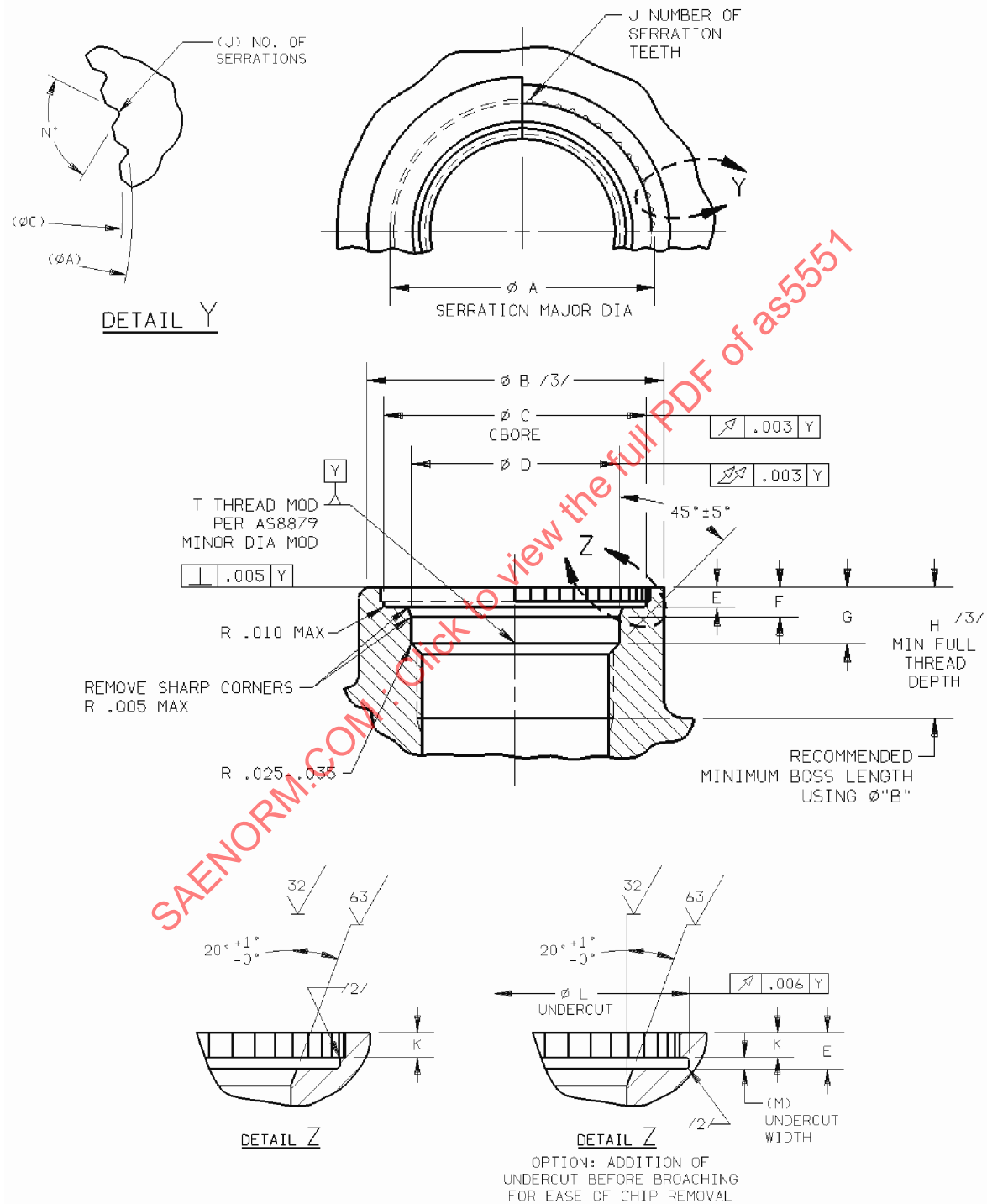
FIGURE 3 - Port
