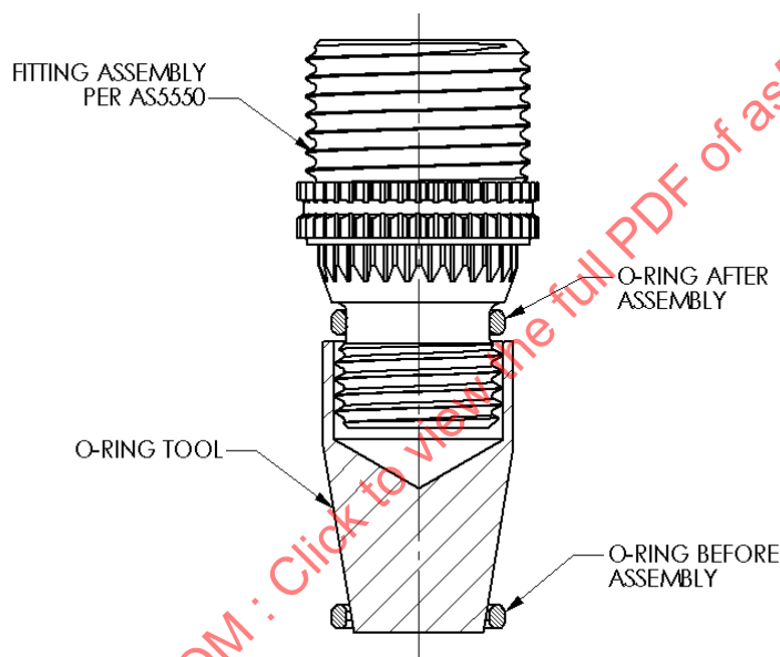
FIGURE 4 - O-ring Installation
