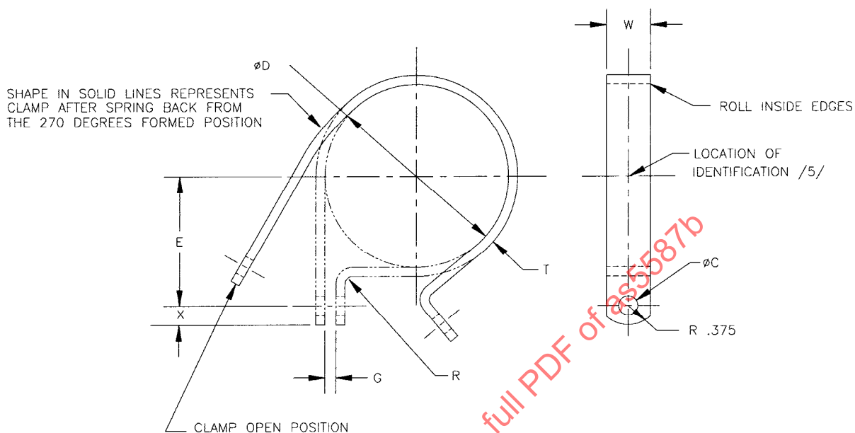
FIGURE 1 - CLAMP
