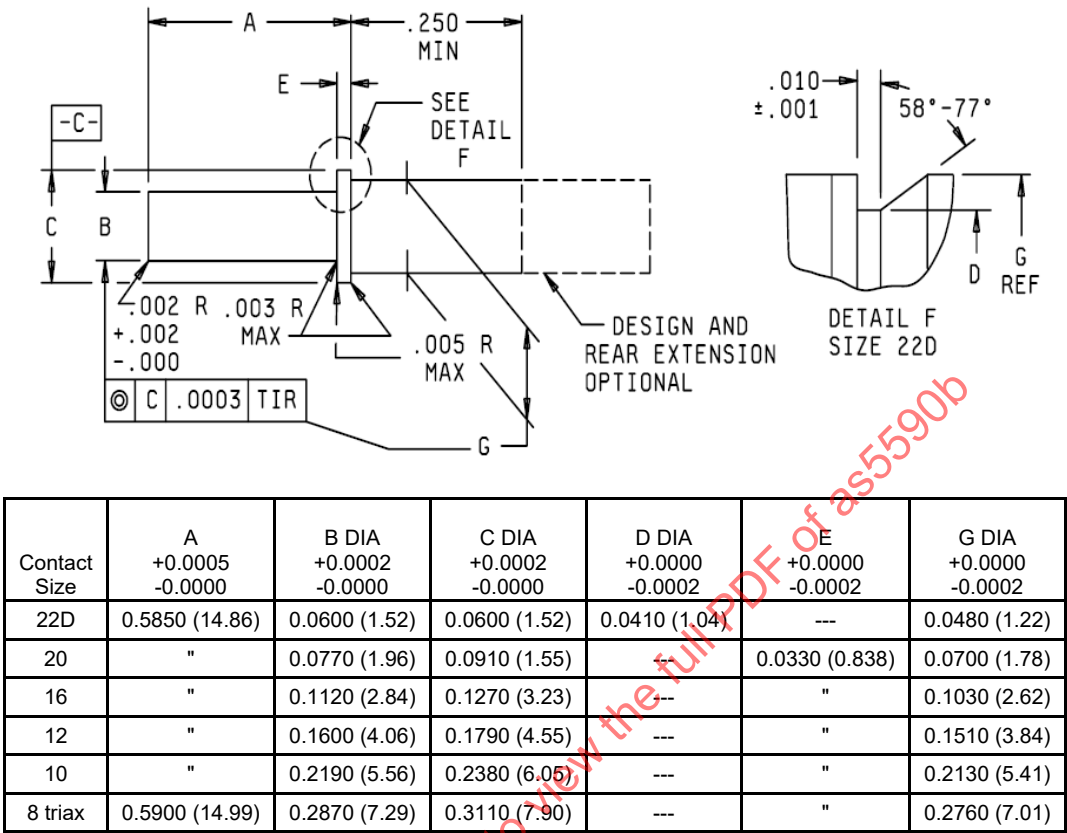
FIGURE 5 - TEST GAUGE, SOCKET, GAUGE LOCATION
