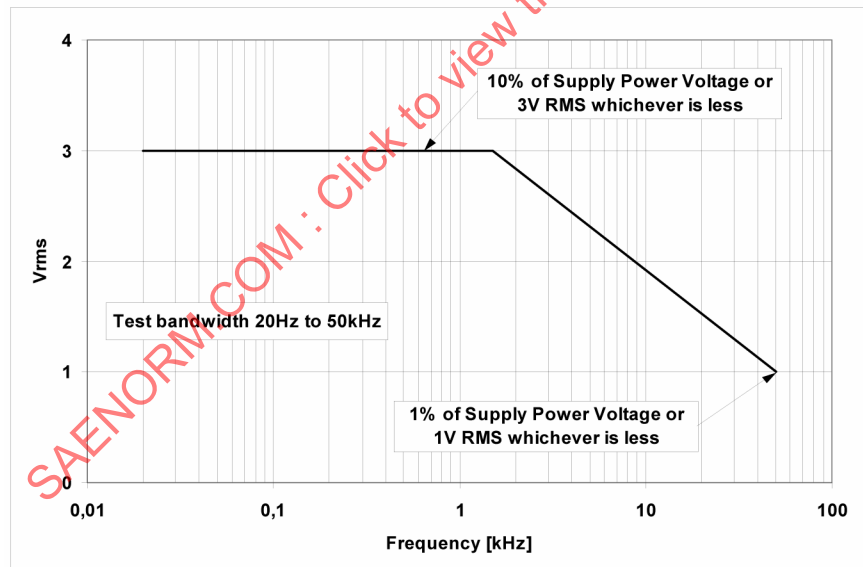
FIGURE 52 - Limits for Conducted Susceptibility, Power Leads
