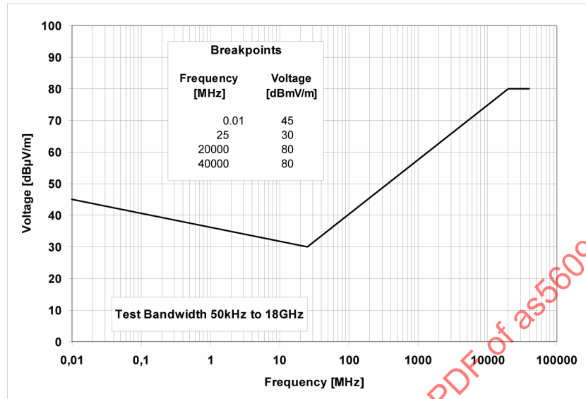
FIGURE 51 - Limits for Radiated Emission, Electric Fields
