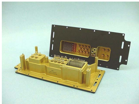
FIGURE 6 - Quadrax PCB Version Installed in ARINC 600 Style Connector
