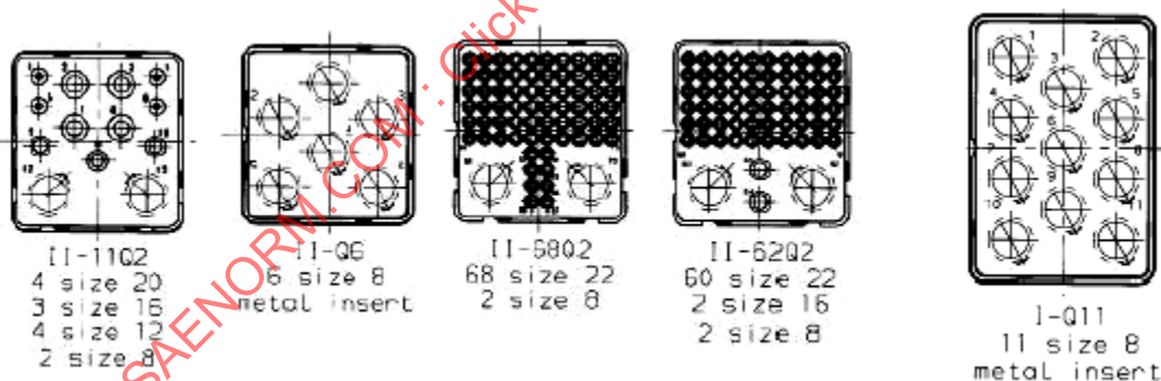
FIGURE 5 - Example of ARINC 600 Style Inserts with #8 Contacts
