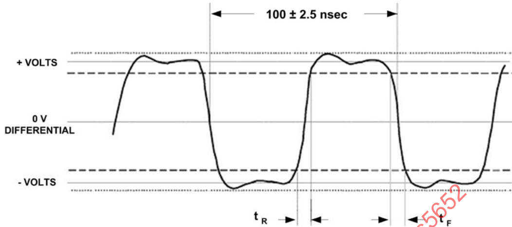
FIGURE 12 - Output Waveform
