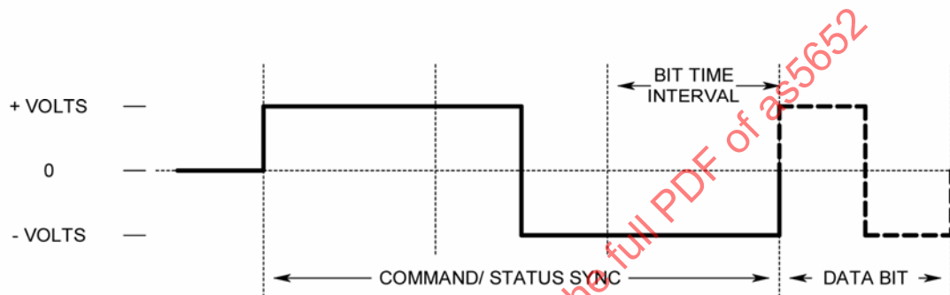
FIGURE 6A - Command and Status Sync Waveform
