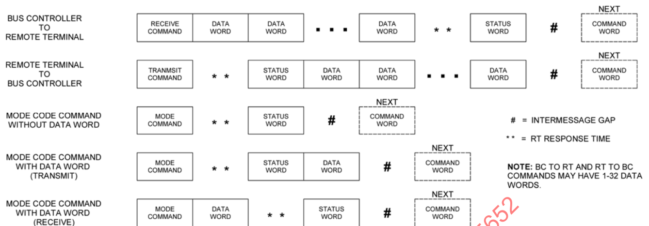
FIGURE 6 - Information Transfer Formats
