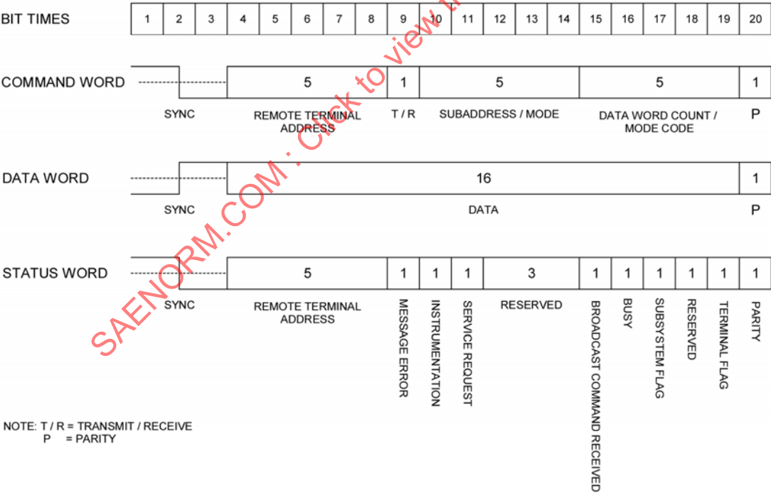
FIGURE 4 - Word Formats
