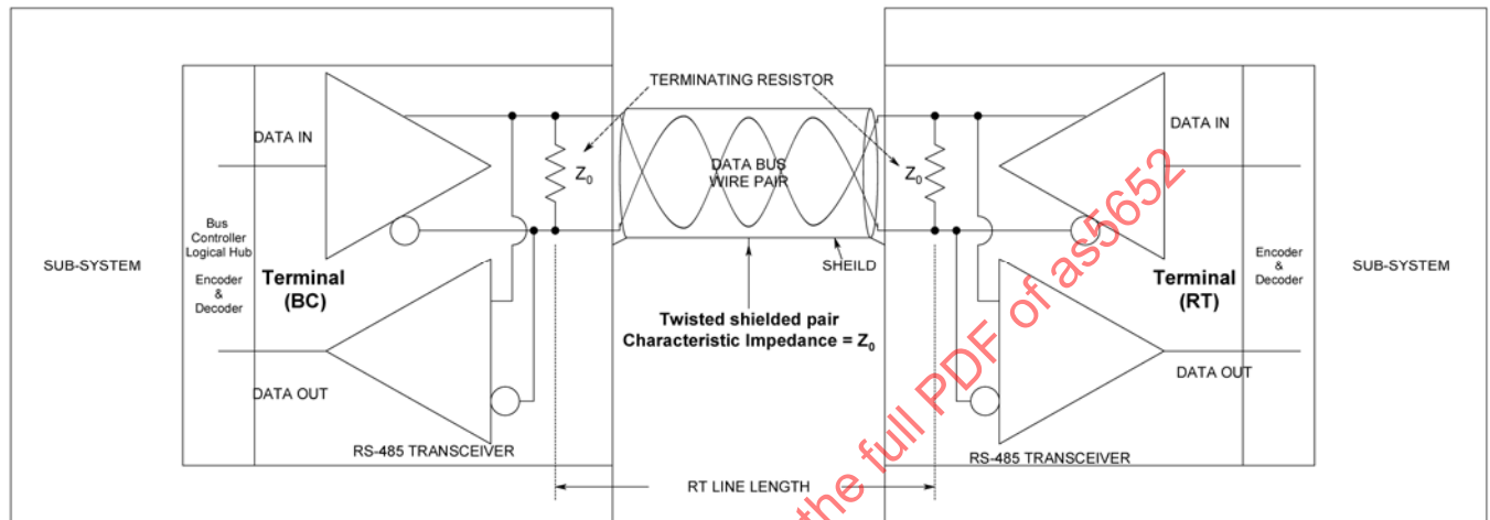
FIGURE 9 - Example Implementation of BC to RT Interface Line Cable
