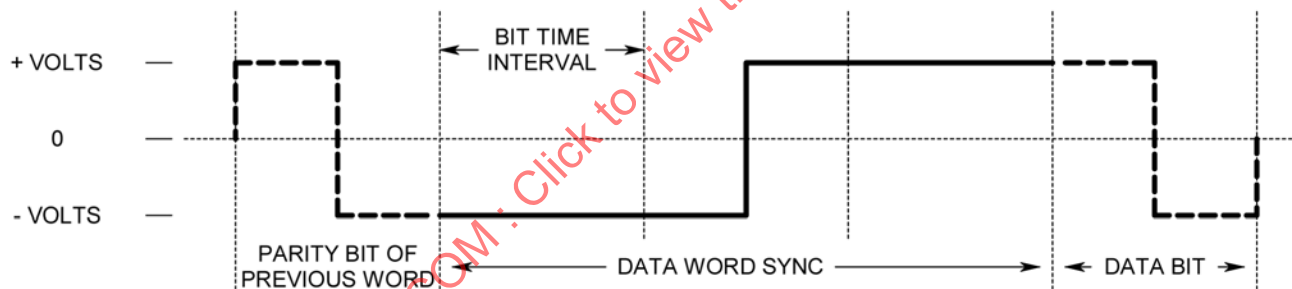
FIGURE 5B - Data Word Sync
