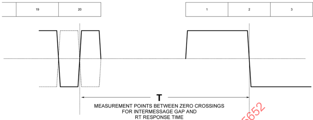
FIGURE 8 - Intermessage Gap and RT Response Time
