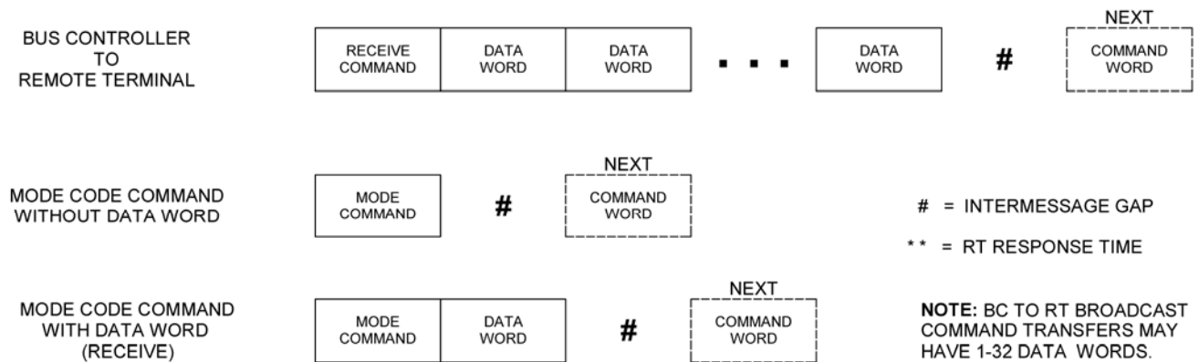
FIGURE 7 - Broadcast Information Transfer Formats
