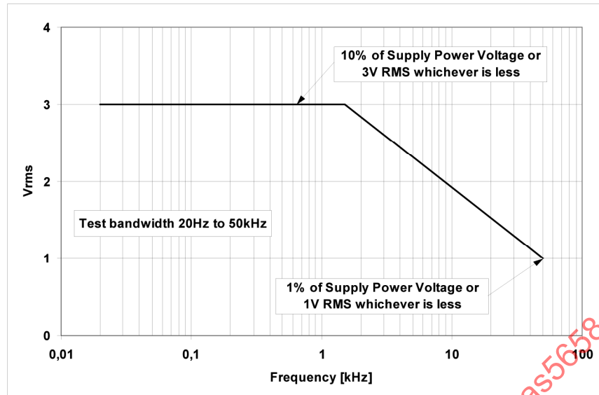
FIGURE 45 – LIMITS FOR CONDUCTED SUSCEPTIBILITY, POWER LEADS
