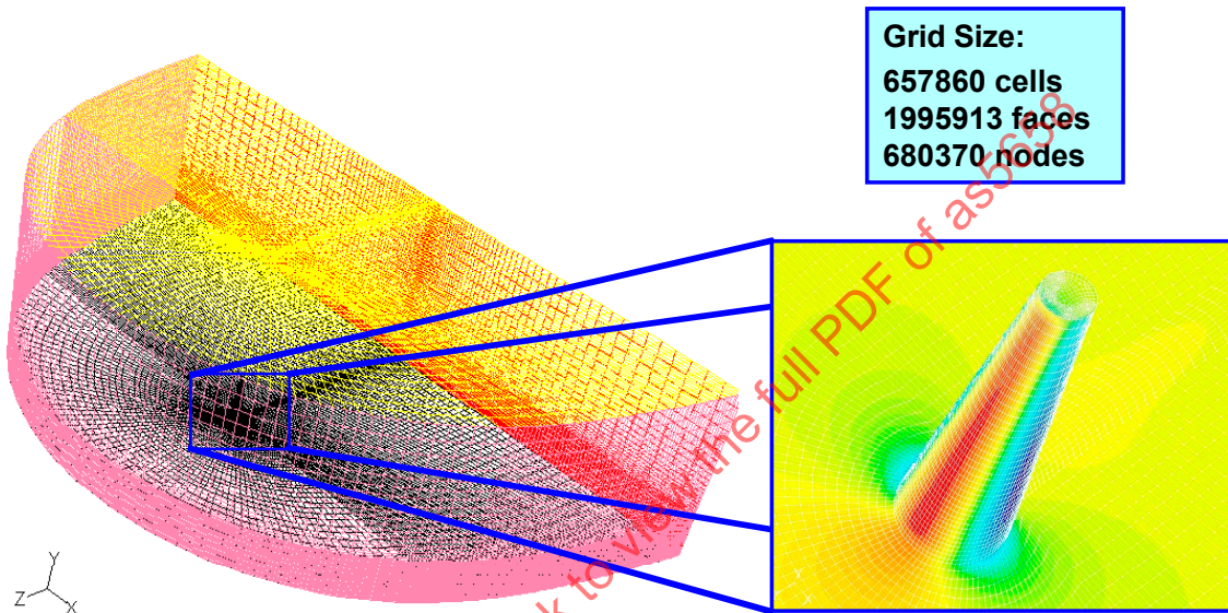
FIGURE 29 – COMPUTATIONAL FLUID DYNAMIC CONTROL VOLUME
