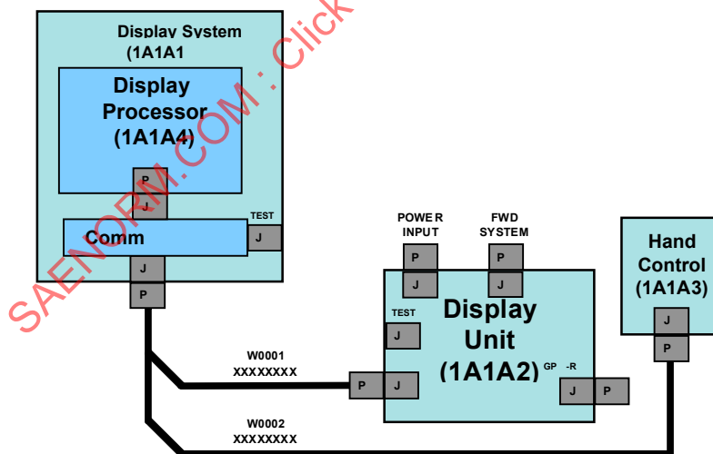
FIGURE 13 – DISPLAY SUBSYSTEM INTERCONNECTS
