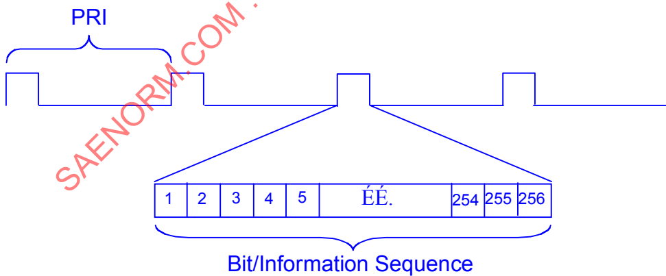
FIGURE 57 – PRI AND INFORMATION SEQUENCE
