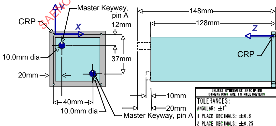
FIGURE 7 – SUBSYSTEM CONNECTOR INTERFACE (PLATFORM SIDE)
