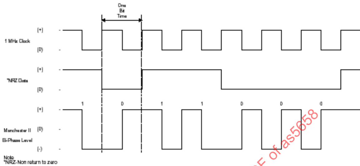
FIGURE 22 – DATA ENCODING
