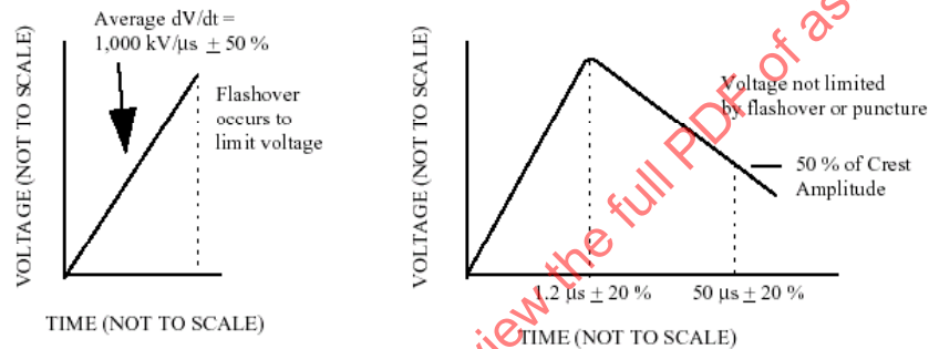
FIGURE 52 – LIGHTNING DIRECT EFFECTS ENVIRONMENT
