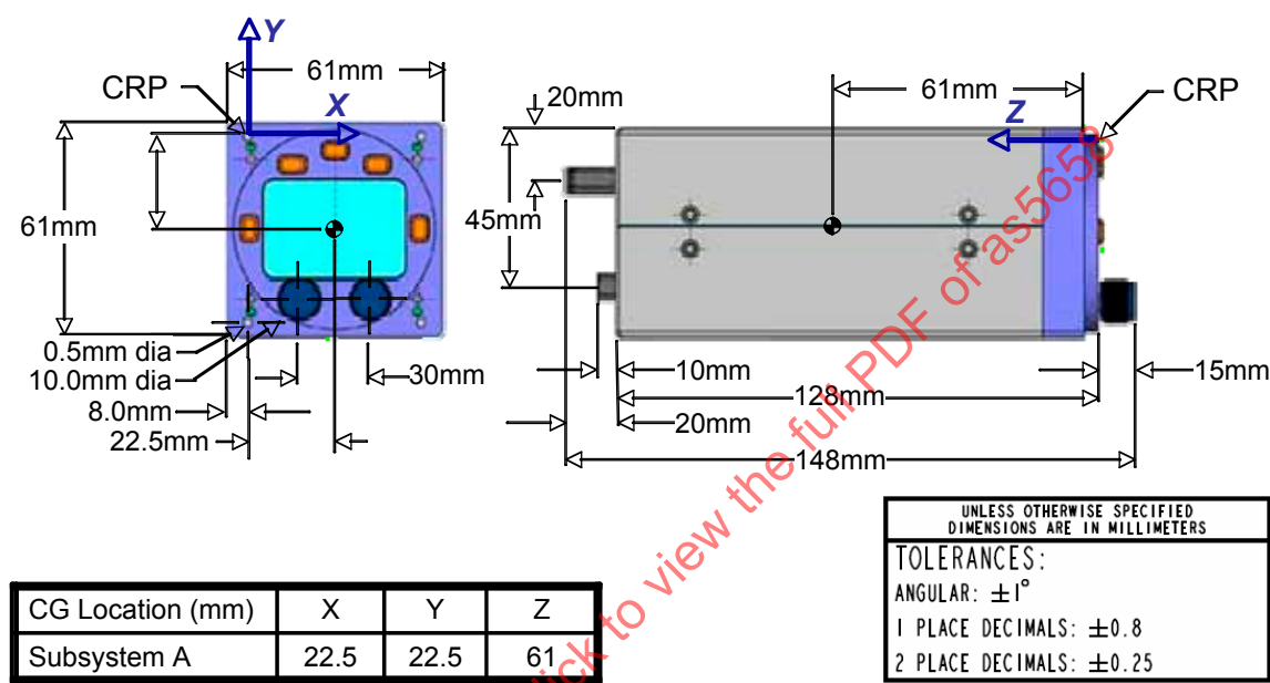
FIGURE 5 – CENTRE OF GRAVITY LOCATION
