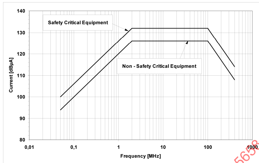
FIGURE 47 – LIMITS OF CURRENT INJECTED INTO A CABLE DURING TEST
