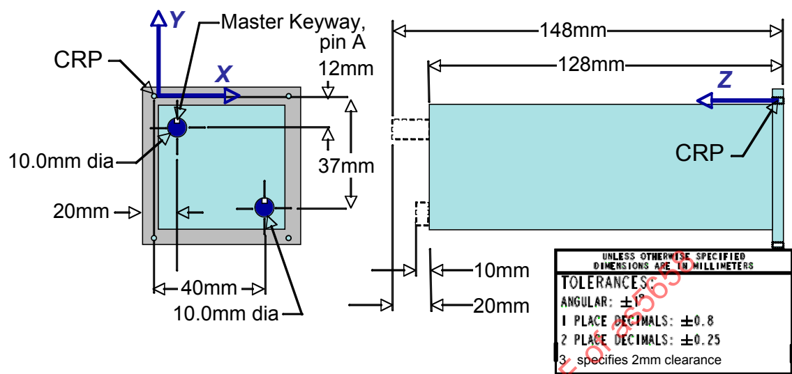
FIGURE 10 – CLEARANCE ENVELOPE FOR SUBSYSTEM INSTALLATION
