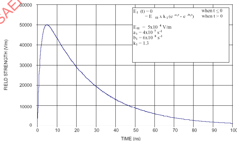
FIGURE 51 – FREE-FIELD EMP ENVIRONMENT
