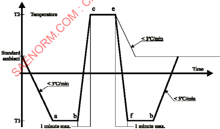
FIGURE 35 – TEMPERATURE SHOCK
