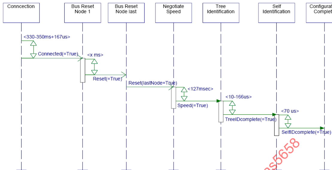
FIGURE 4 – SEQUENCE OF EVENTS: BUS CONFIGURATION
