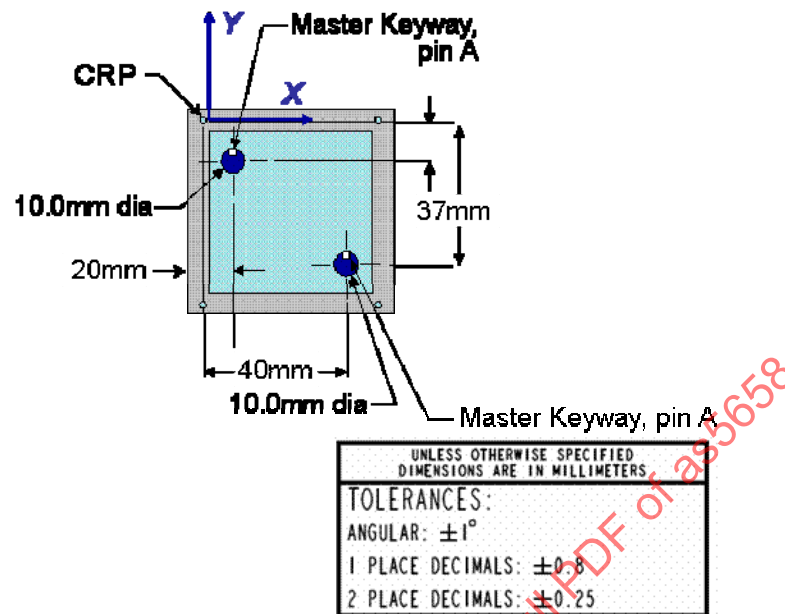
FIGURE 9 – PLATFORM SUBSYSTEM MOUNTING INTERFACE
