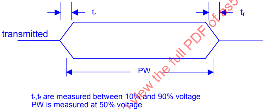
FIGURE 56 – DATA LINK PULSE CHARACTERISTIC
