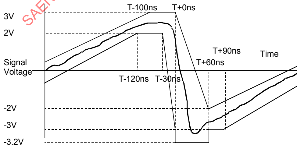
FIGURE 20 – TIME DOMAIN TEMPLATE. ONE PULSE
