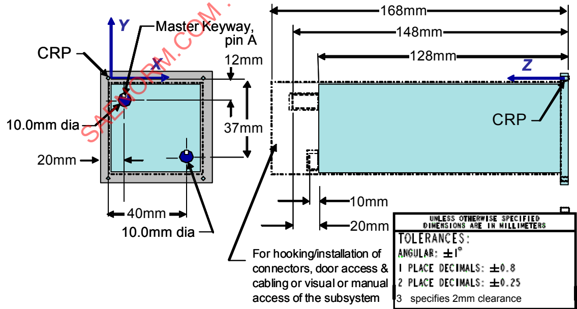
FIGURE 11 – CLEARANCE ENVELOPE FOR SUBSYSTEM PREPARATION/SETTING
