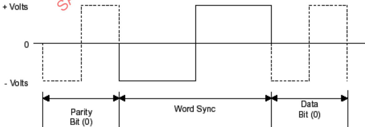
FIGURE 24 – DATA SYNC WAVEFORM
