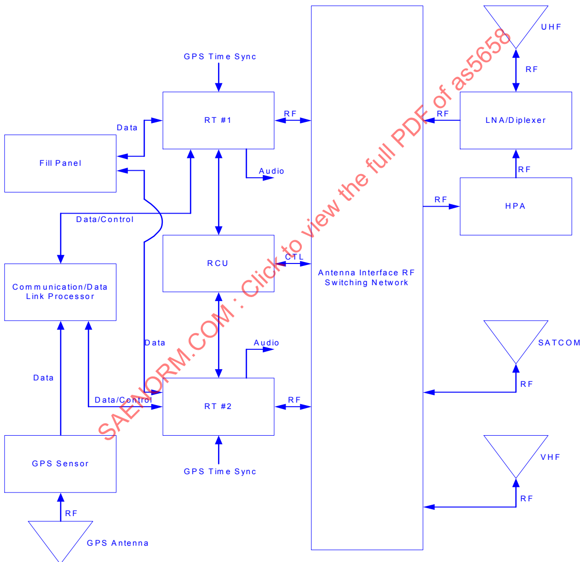
FIGURE 55 – COMMUNICATION SYSTEM ARCHITECTURE LAYOUT
