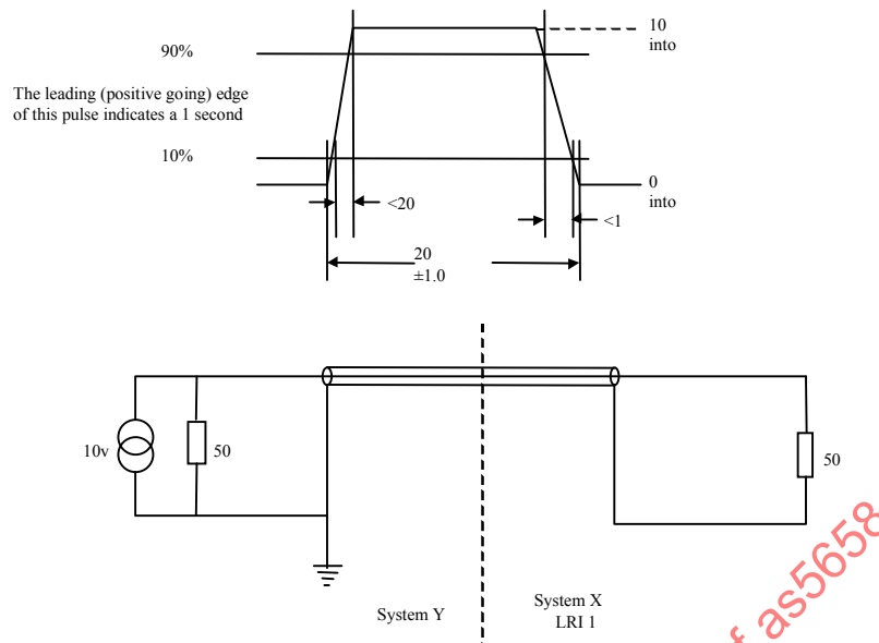
FIGURE 19 – ANALOGUE SIGNAL 1 DEFINITION
