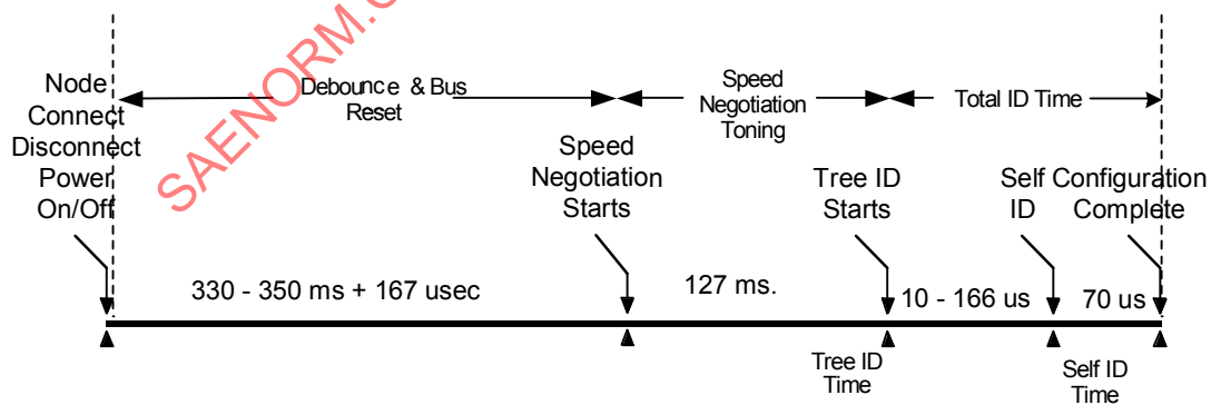
FIGURE 5 – BUS CONFIGURATION TIMELINE
