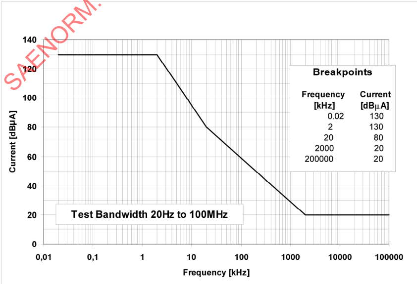
FIGURE 42 – CONDUCTED EMISSIONS, LIMITS FOR POWER LEADS/CONTROL AND SIGNAL LINES
