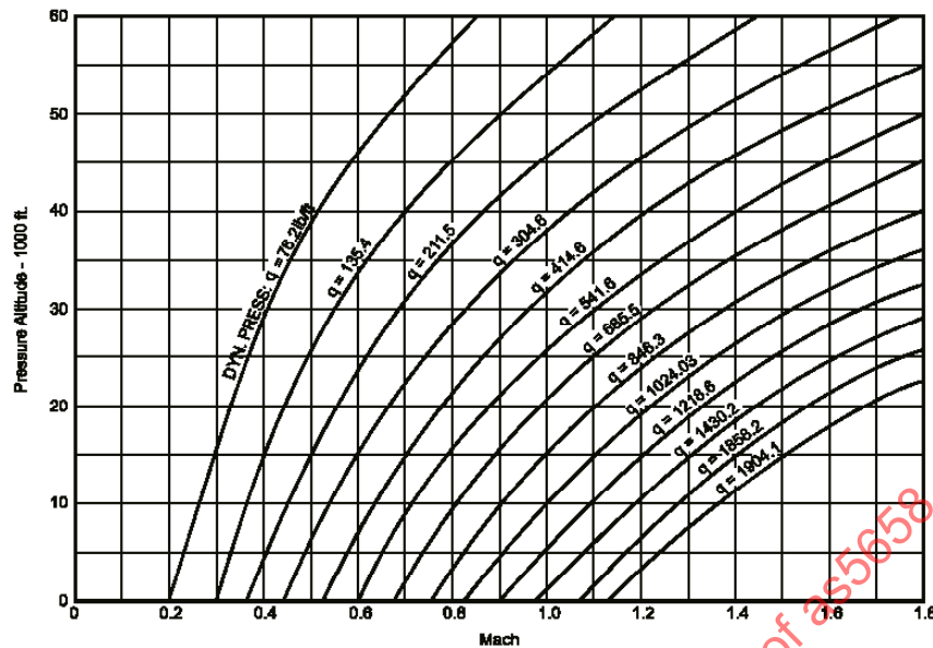
FIGURE 34 – DYNAMIC PRESSURE AS FUNCTION OF MACH NUMBER
