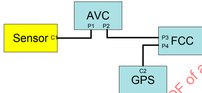
FIGURE 2 – AVIONICS ARCHITECTURE
