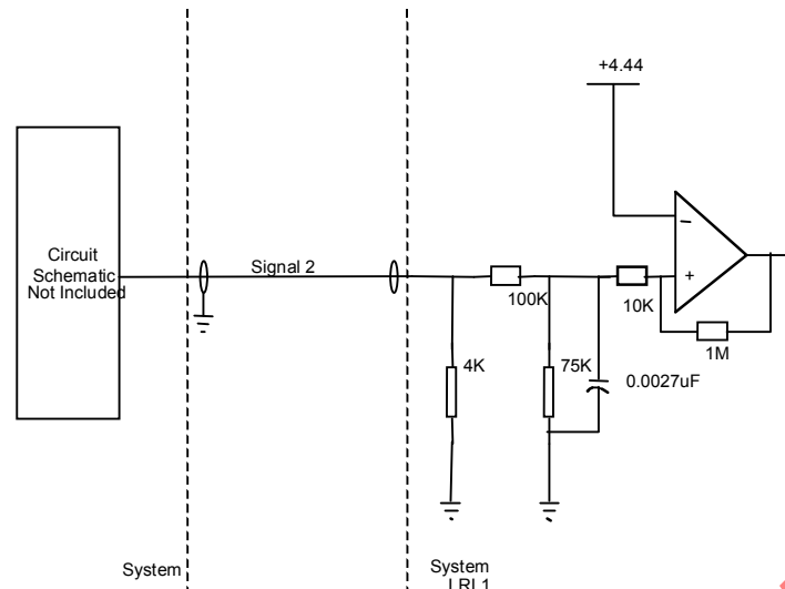
FIGURE 18 – DISCRETE SIGNAL 1 DEFINITION
