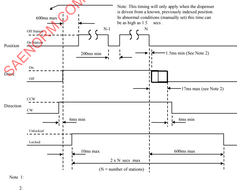
FIGURE 26 – DISPENSER SIGNAL TIMING
