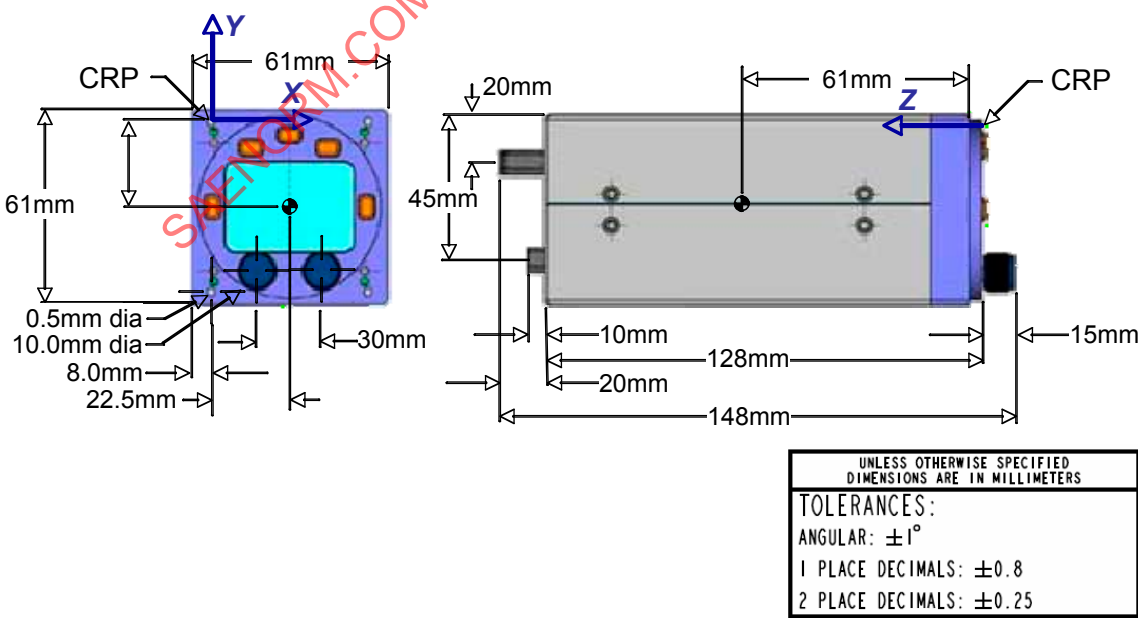
FIGURE 3 – RELATIVE SUBSYSTEM DIMENSIONS
