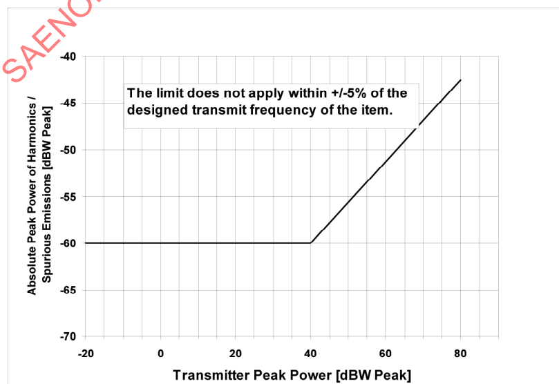
FIGURE 49 – LIMITS OF TRANSMITTER/RECEIVER EMISSIONS
