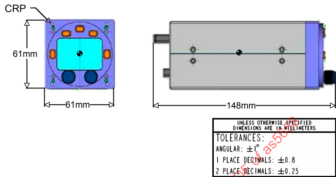
FIGURE 2 – ABSOLUTE SUBSYSTEM DIMENSIONS
