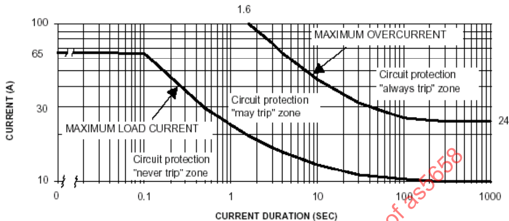
FIGURE 16 – INTERFACE CURRENT LEVEL
