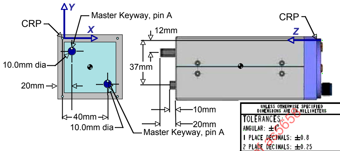
FIGURE 6 – SUBSYSTEM CONNECTOR INTERFACE (SUBSYSTEM SIDE)
