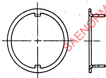
Key washer
