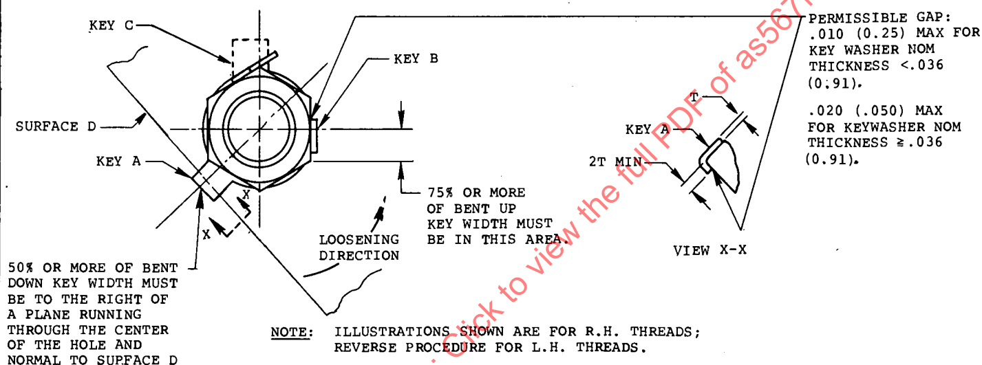
φ FIGURE II-1 KEY WASHER STATIONARY SURFACE LOCK
