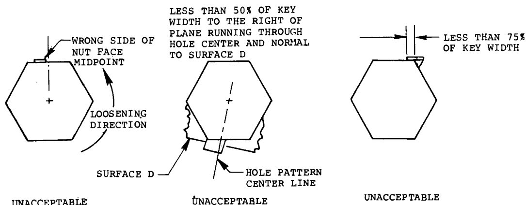
φ FIGURE II-2 UNACCEPTABLE BENT KEY LOCATIONS
