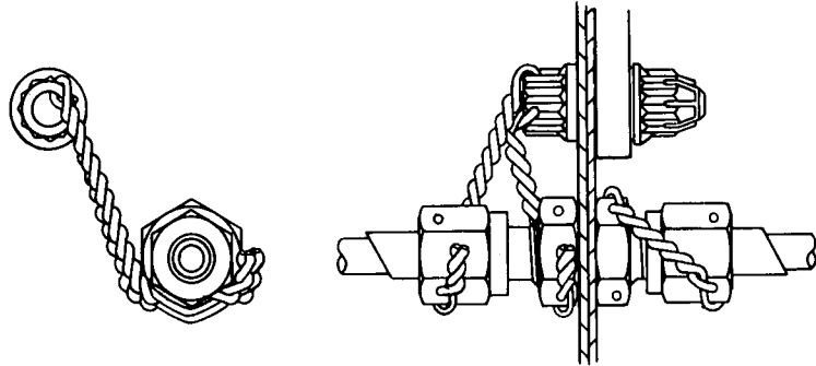
FIGURE I-26 Straight connector (bulkhead type)
