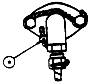
FIGURE 25 - Small coupling nuts or those made of soft material may be wired as shown to lessen possibility of wire breaking or tearing out.
