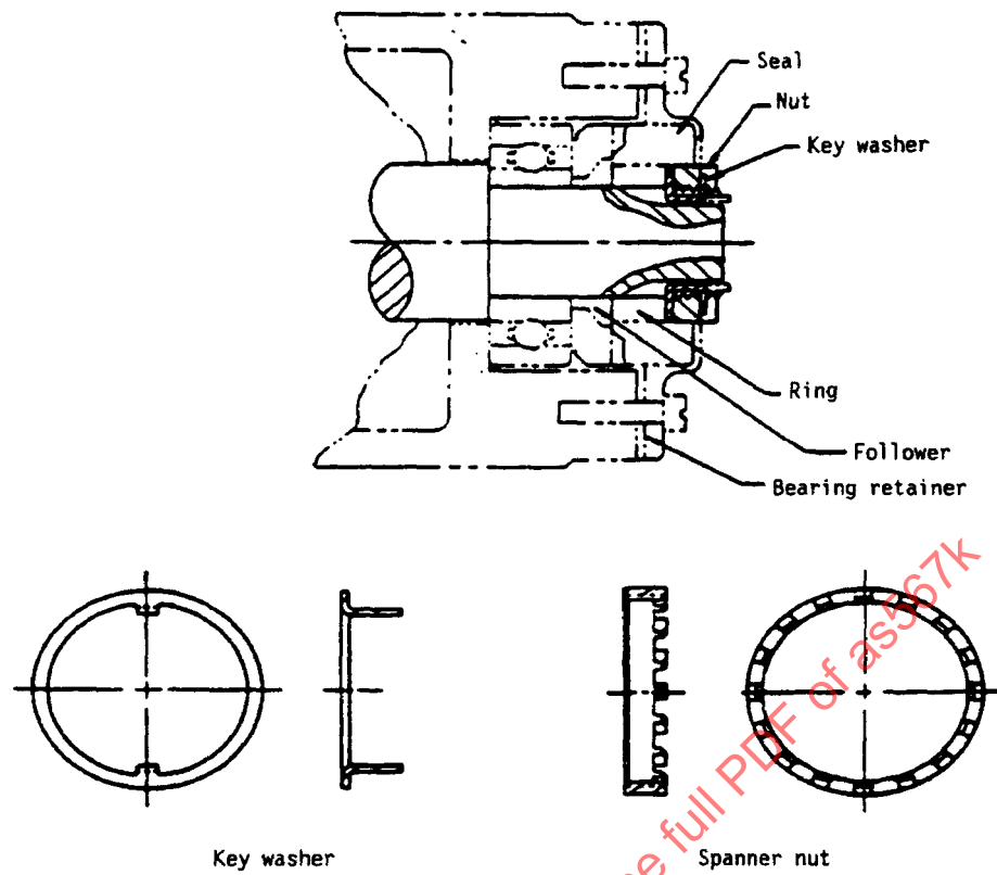
Figure 44 - Key washers and spanner nuts
