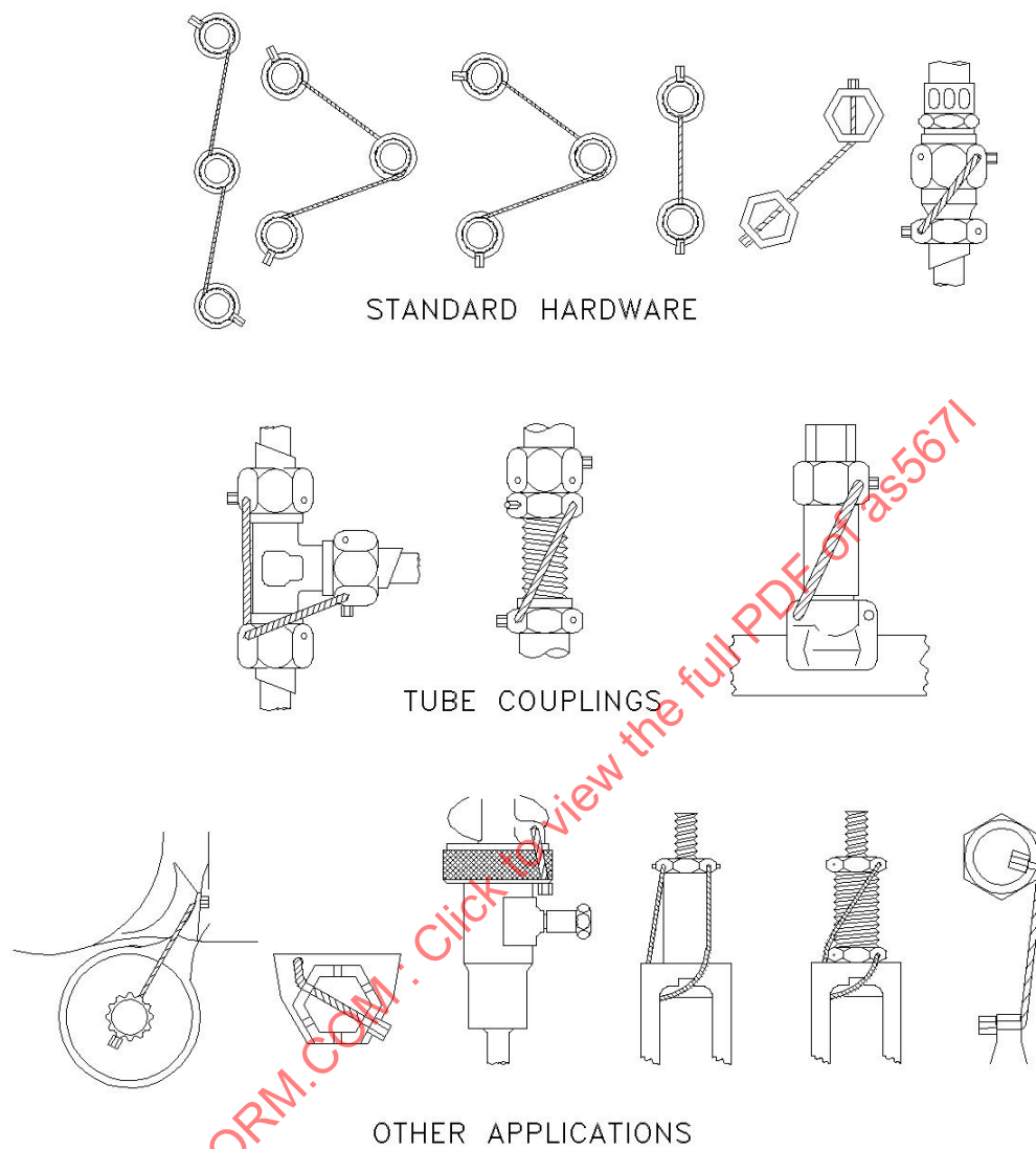
Figure 33 - Safety-cable, typical installation (standard hardware)
