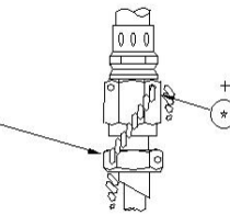
FIGURE 22 – Correct method for wiring the coupling nut on flexible line to the straight connector braced on rigid tube.
