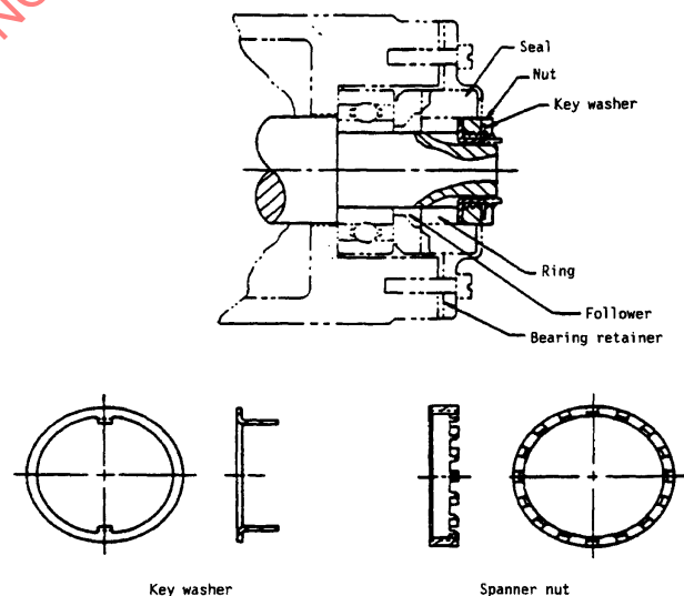
Figure 42 - Key washers and spanner nuts
