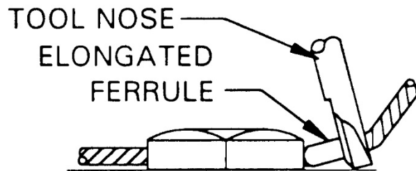
Figure 34 - Low profile installations (using the AS3618 or AS3619 elongated ferrules)
