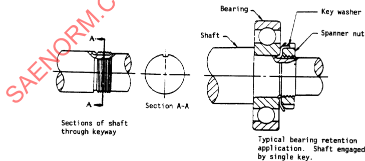
Figure 40 - Typical single key bearing retention application
