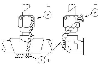
FIGURE 23 – Fittings incorporating wire lugs shall be wired as shown
