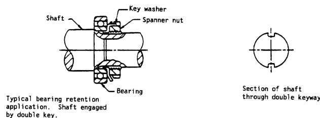
Figure 41 - Typical double key bearing retention application
