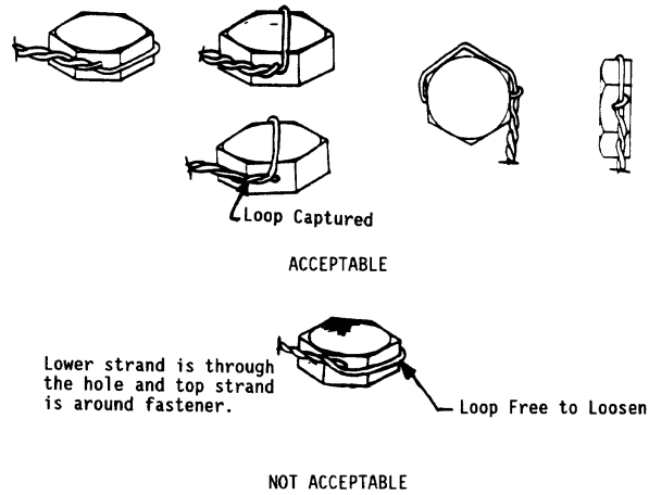
Figure 4 - Upper and lower strand orientation
