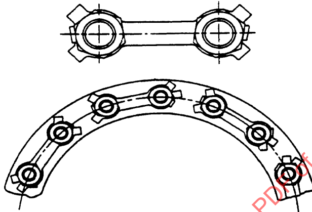
Figure 39 - View showing split line nuts locked with multiple key washers
