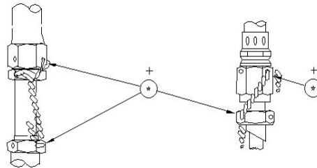
FIGURE 22 – Correct method for wiring the coupling nut on flexible line to the straight connector braced on rigid tube.
