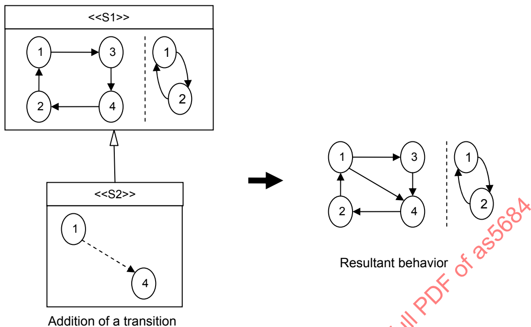
FIGURE 21 - ADDITION OF FEATURES - TRANSITION
