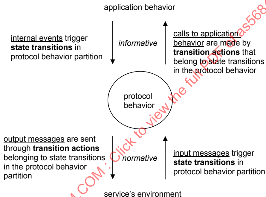
FIGURE 16 - SEPARATION OF PROTOCOL BEHAVIOR FROM APPLICATION BEHAVIOR
