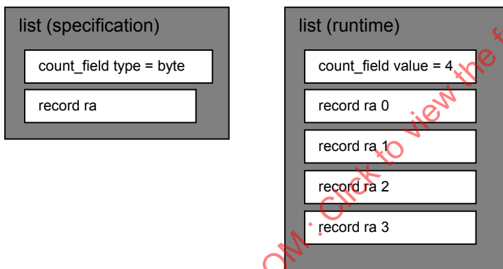
FIGURE 8 - LIST – A VARIABLE SIZED SEQUENCE OF SIMPLE OR COMPOSITE FIELDS OF THE SAME TYPE
