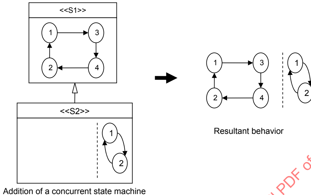
FIGURE 20 - ADDITION OF FEATURES – CONCURRENT STATE MACHINES
