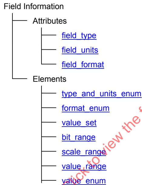
FIGURE 14 - FIELD INFORMATION ATTRIBUTES AND ELEMENTS - PROVIDE INFORMATION ABOUT ENCODED DATA
