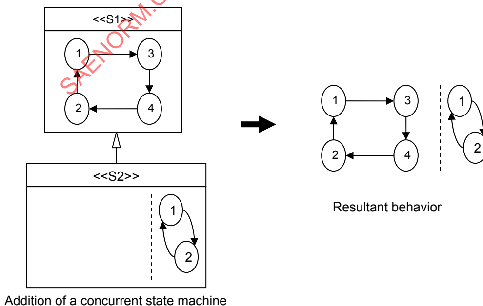
FIGURE 20 - ADDITION OF FEATURES – CONCURRENT STATE MACHINES
