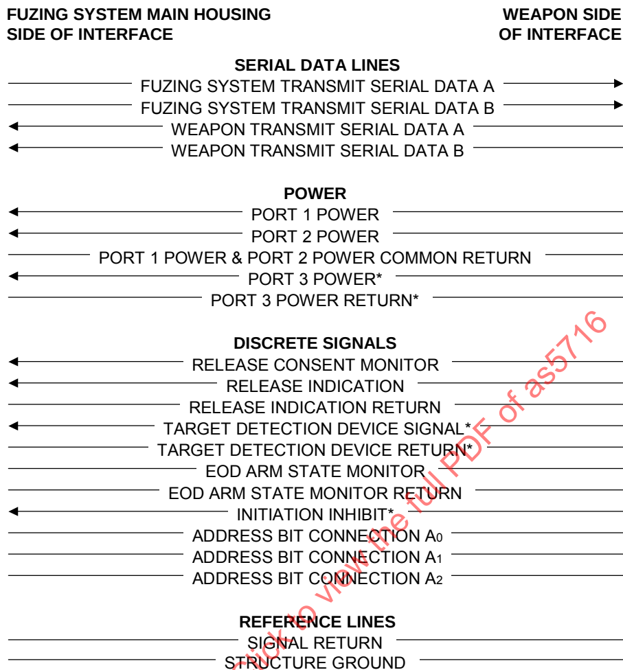
FIGURE 2 - CLASS 2 FUZING SYSTEM INTERFACE CONNECTIONS AND DIRECTION OF SIGNAL FLOW
