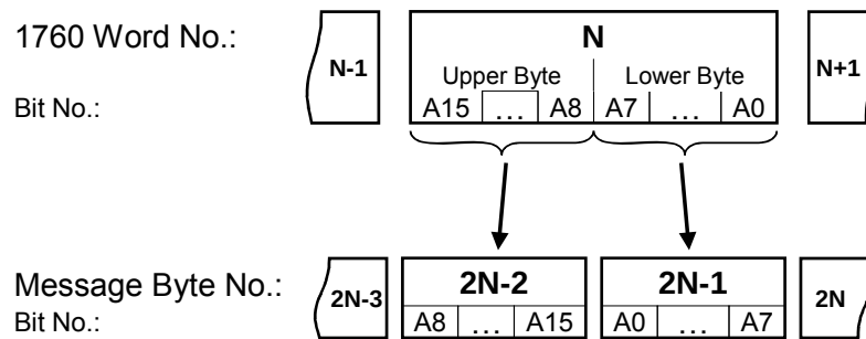
FIGURE 7 - BIT TRANSFER ORDER FOR MIL-STD-1760 FUZING SYSTEM SETTING DATA
