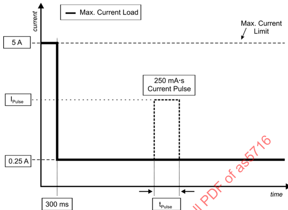
FIGURE 6 - PORT 2 POWER CURRENT LIMITS
