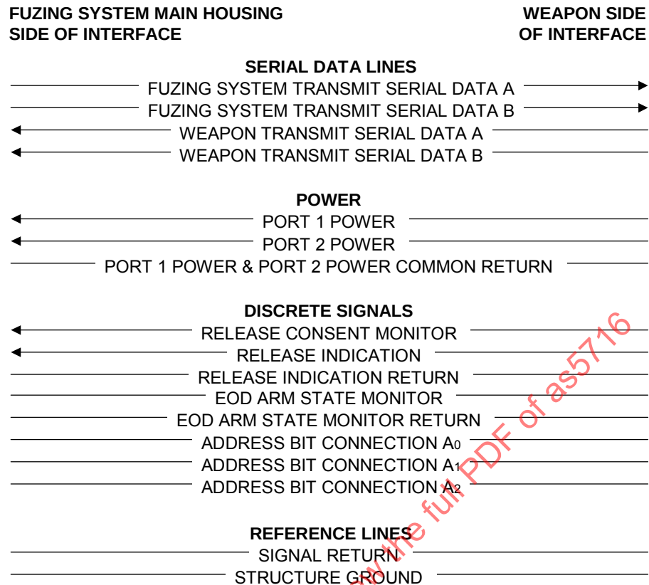
FIGURE 1 - CLASS 1 INTERFACE CONNECTIONS AND DIRECTION OF SIGNAL FLOW
