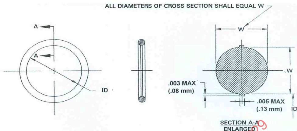
FIGURE 1 – O-RING DIMENSIONS REFERENCE FOR TABLE 1. WIDTH (W) AND INSIDE DIAMETER (ID)
