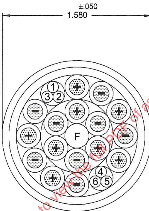
FIGURE 1 - AS5756/7 CABLE
