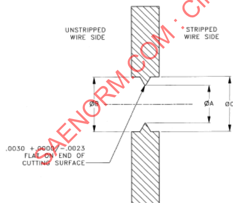
FIGURE 2- BLADE DIES (SEE TABLE 2 AND AS5768)
