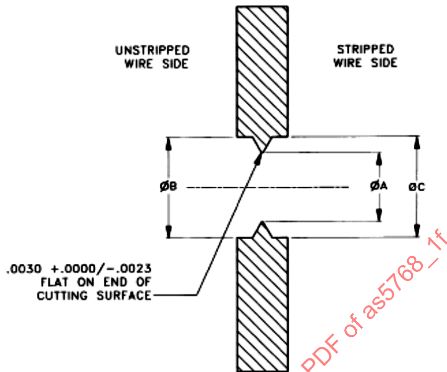
FIGURE 3 - BLADE DIES (SEE TABLE 2 AND AS5768)
