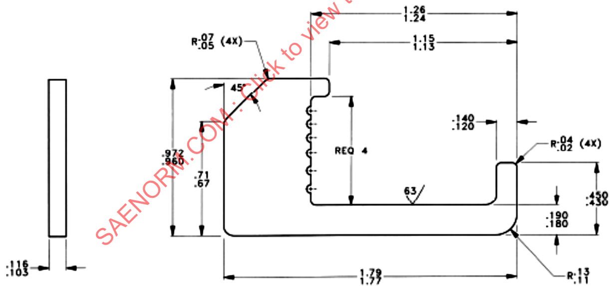
FIGURE 3 - BLADE DIES (SEE TABLE 2 AND AS5768)
