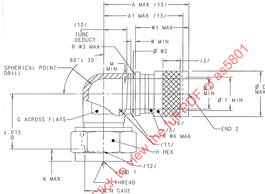
FIGURE 1 - ELBOW, 90 DEGREE, FEMALE FLARELESS, SWAGE
