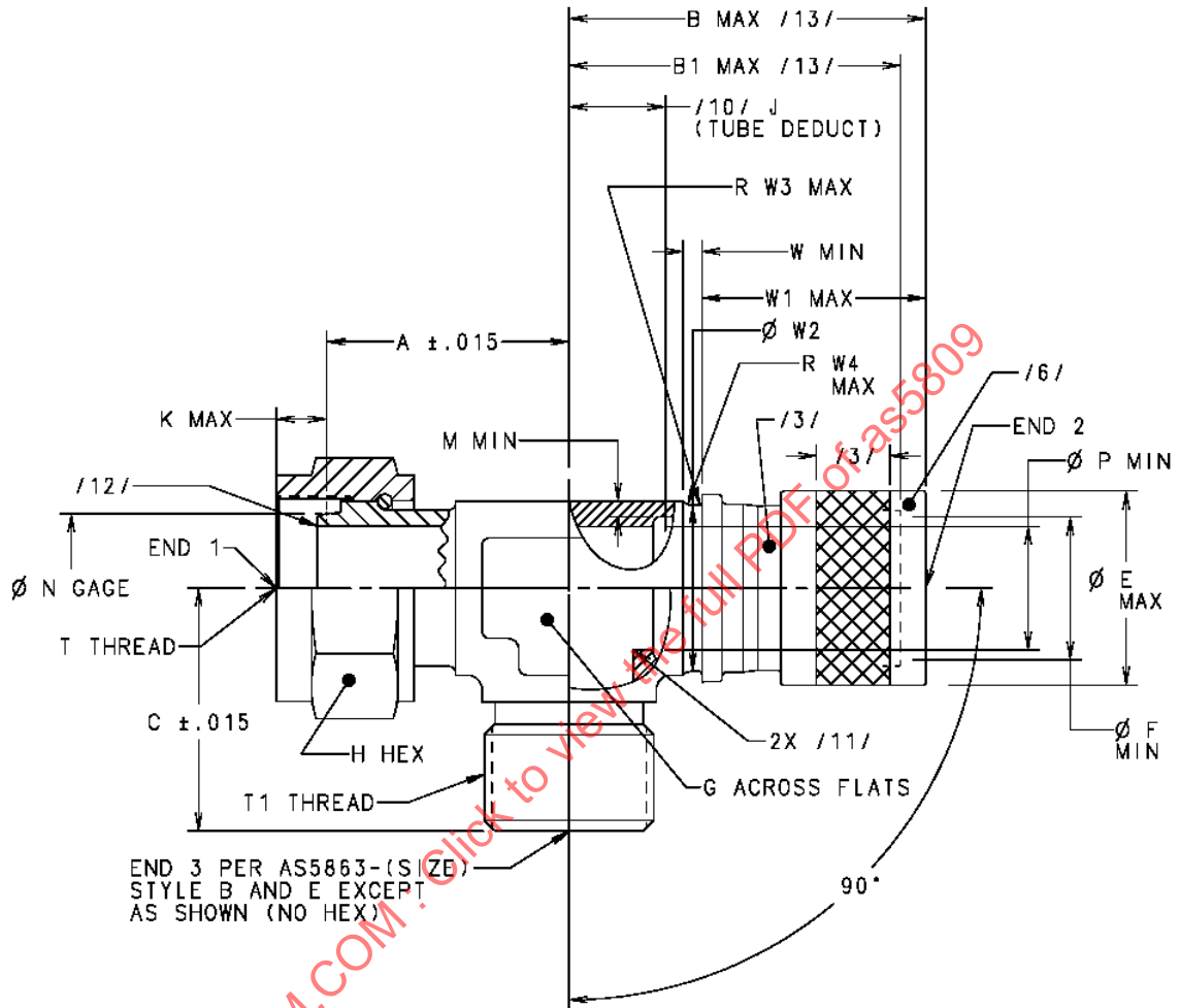
FIGURE 1 - TEE, FEMALE FLARELESS, MALE FLARELESS, SWAGE
