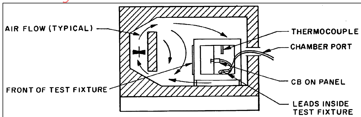
Figure 4D - Typical chamber installation
