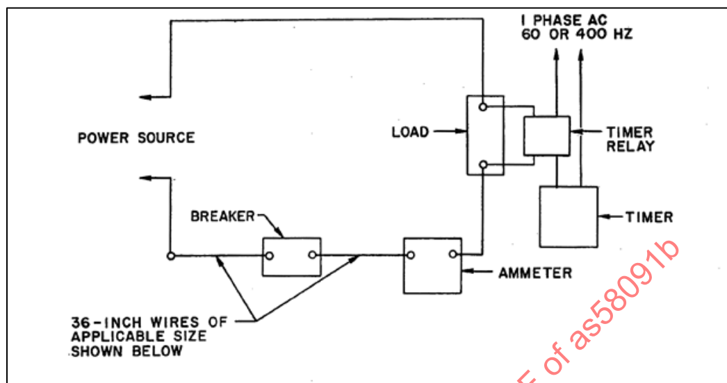
Figure 2 - Calibration test circuit
