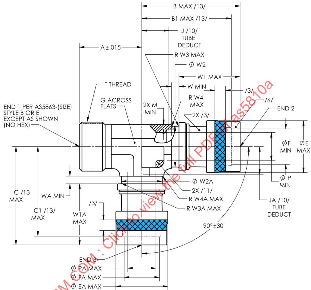
FIGURE 1 - FITTING ASSEMBLY, TEE, MALE FLARELESS ON THE RUN, AXIALLY SWAGED ON THE RUN AND THE BRANCH
