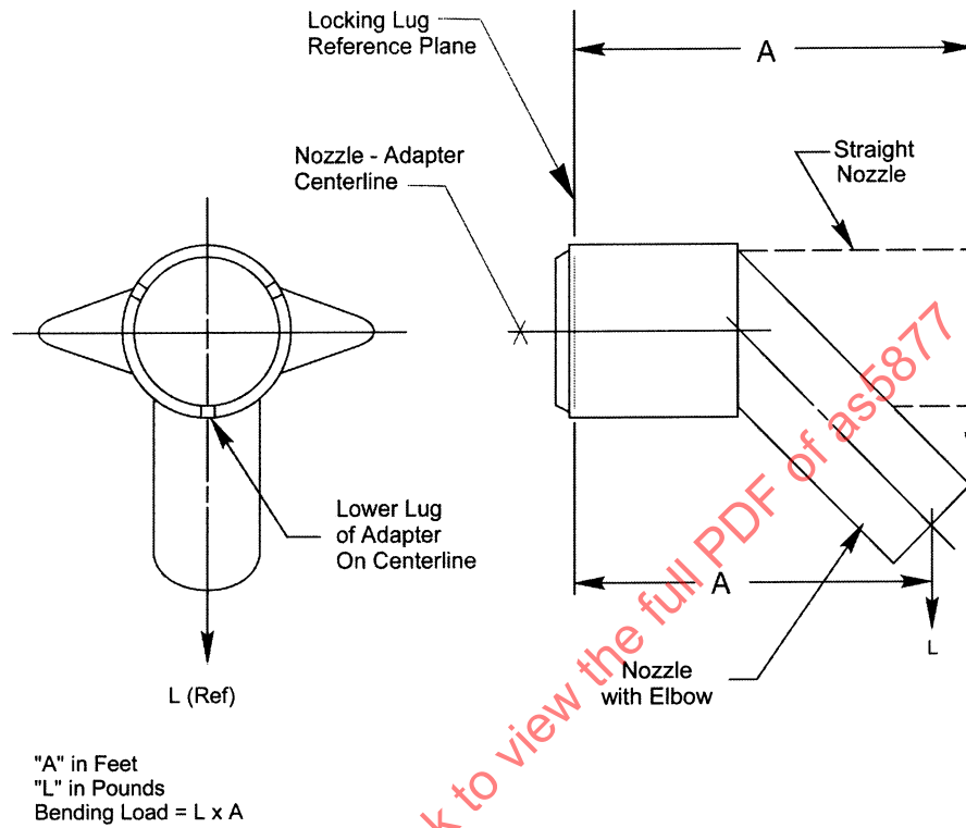
FIGURE 2 - Strength Test Setup
