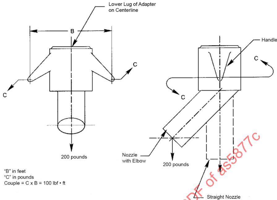
Figure 3 - Swivel strength test setup
