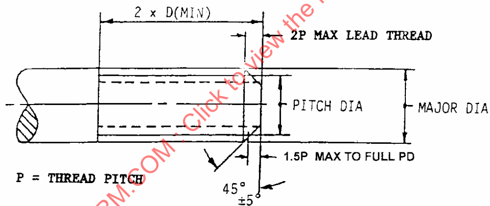
FIGURE E2 - Minimum Material Bolt or Stud
