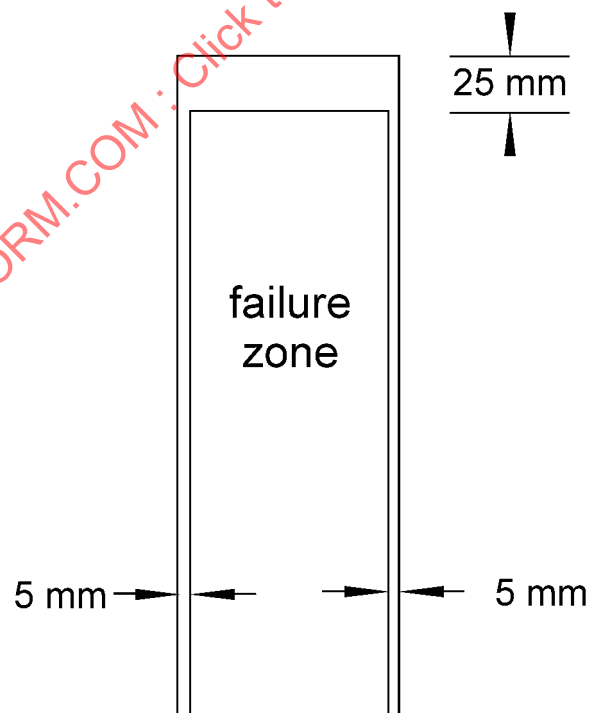
FIGURE 1 - LINE MARKINGS ON THE TEST PLATE TO DELINEATE THE FAILURE ZONE
