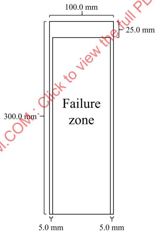
Figure 1 - Line markings on the test plate to delineate the failure zone ( \pm 0.5 mm)
