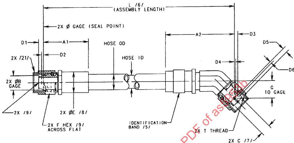
FIGURE 1 - FLARELESS HOSE ASSEMBLY, STRAIGHT TO 45° ELBOW
