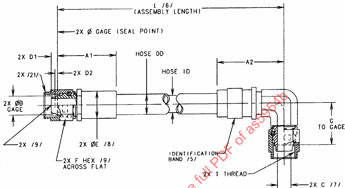
FIGURE 1 - FLARELESS HOSE ASSEMBLY, STRAIGHT TO 90° ELBOW
