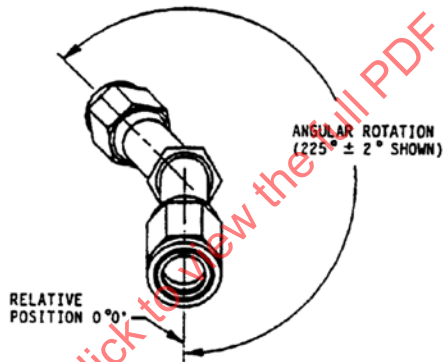
FIGURE 2 - FITTING ORIENTATION /17/
