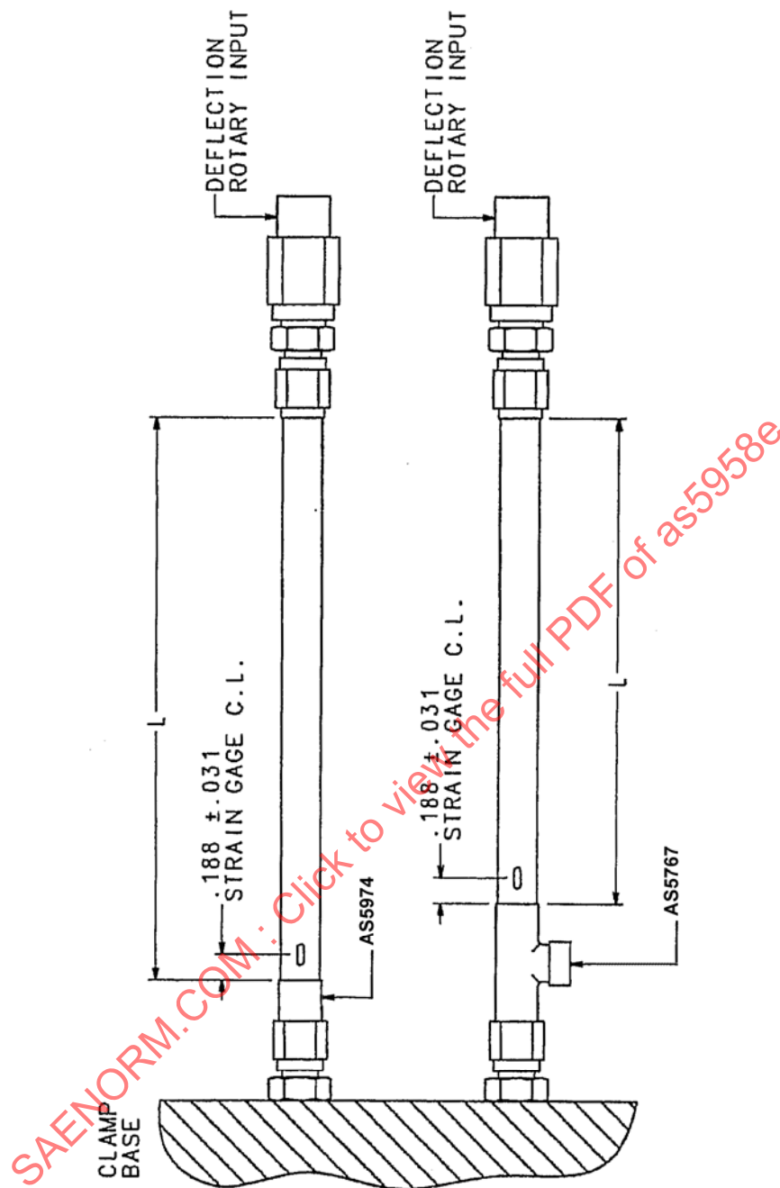
FIGURE 3 - ROTARY IMPULSE TEST SPECIMEN
