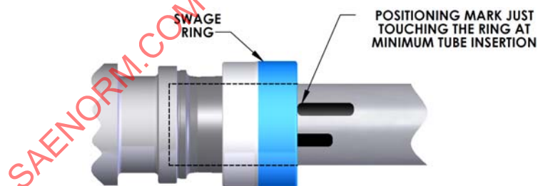
FIGURE 3A - POSITIONING MARK AT MINIMUM TUBE INSERTION
