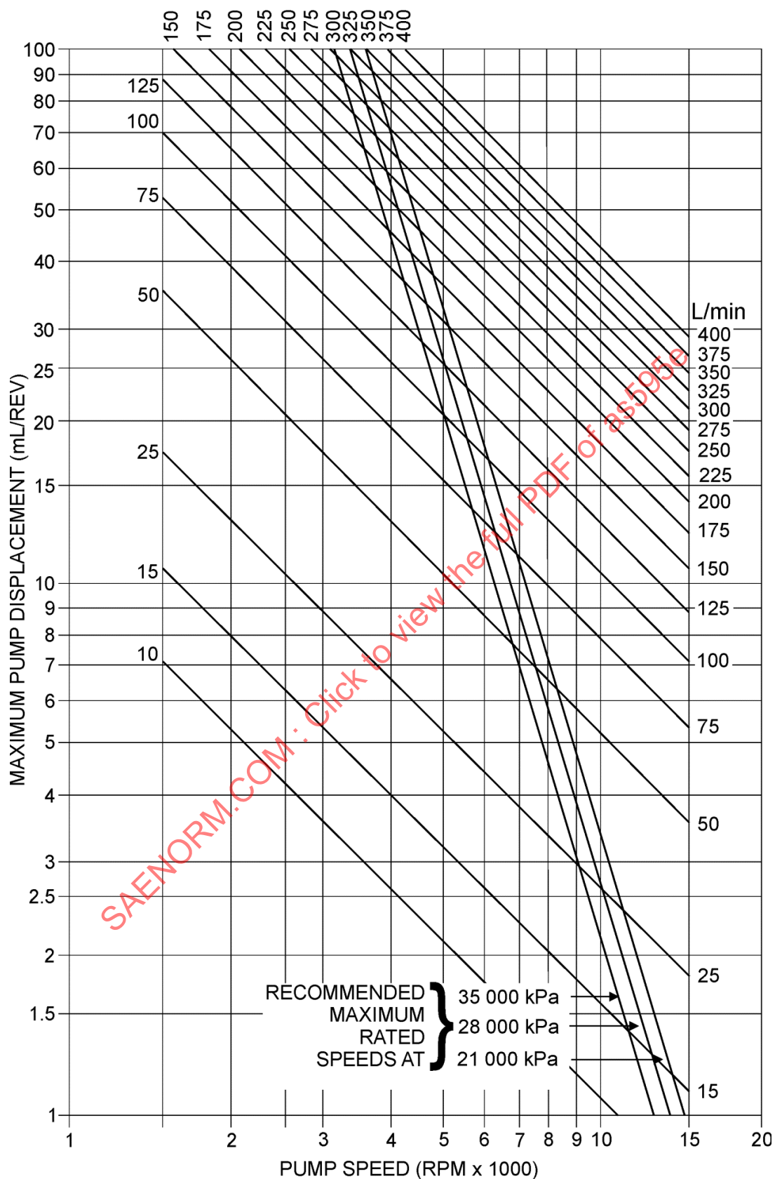
Figure 4B - Nomograph of maximum recommended values for rated speeds against pump displacement (metric units)
