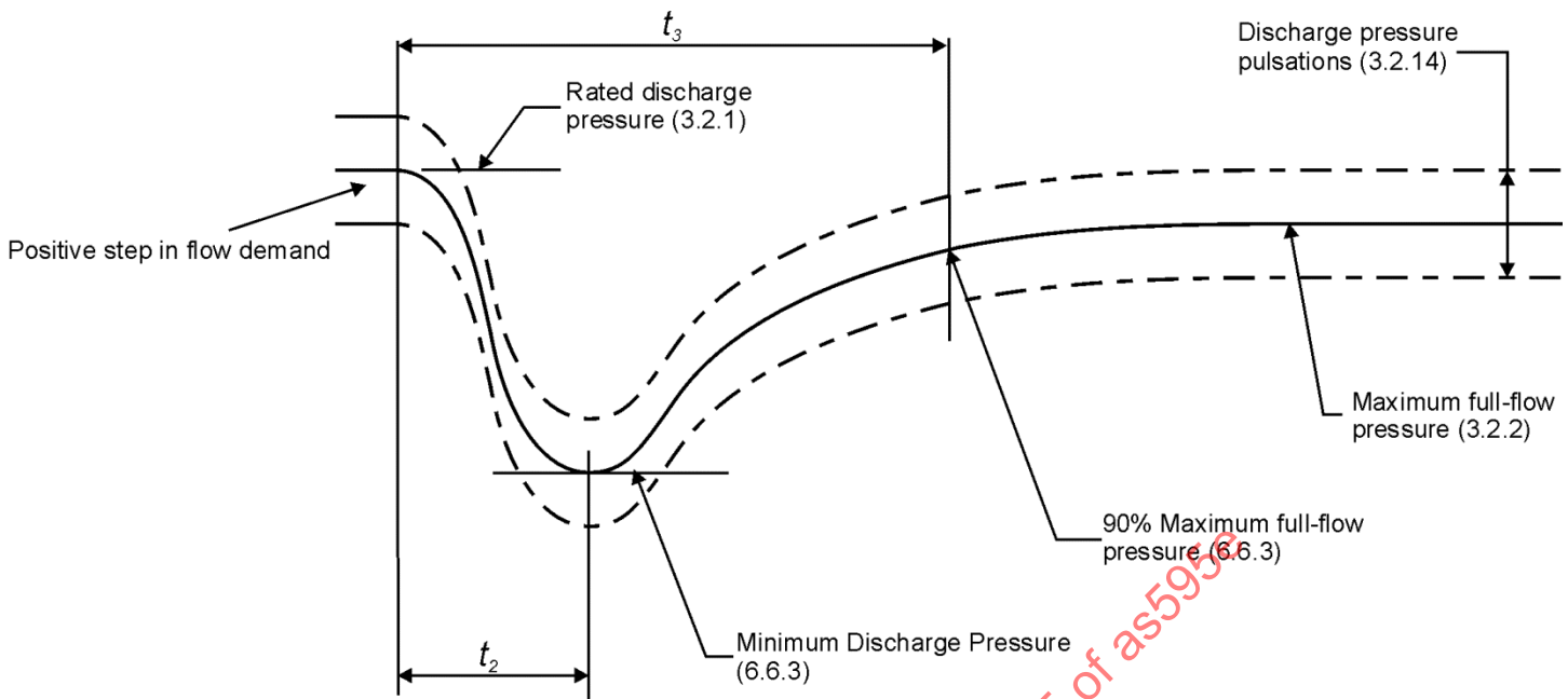
Figure 3 - Typical variation of discharge pressure against time - transient from rated discharge pressure (zero-flow) to maximum full-flow pressure
