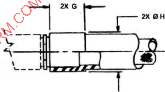
FIGURE 2 - INTEGRAL FIRESLEEVECUFF / 13/
