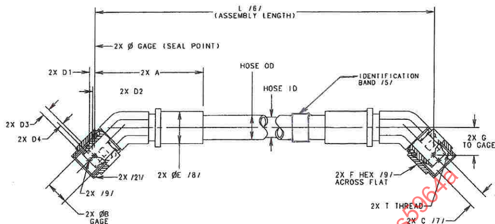
FIGURE 1 - HOSE ASSEMBLY DIMENSIONS
