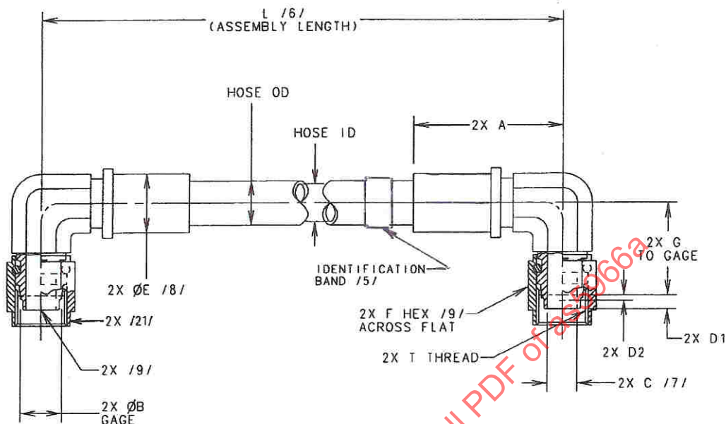
FIGURE 1 - HOSE ASSEMBLY DIMENSIONS
