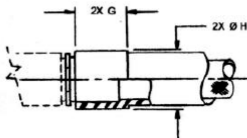
FIGURE 3 - INTEGRAL FIRESLEEVE CUFF /13/
