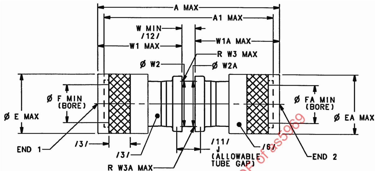
FIGURE 1 - UNION, SWAGE
