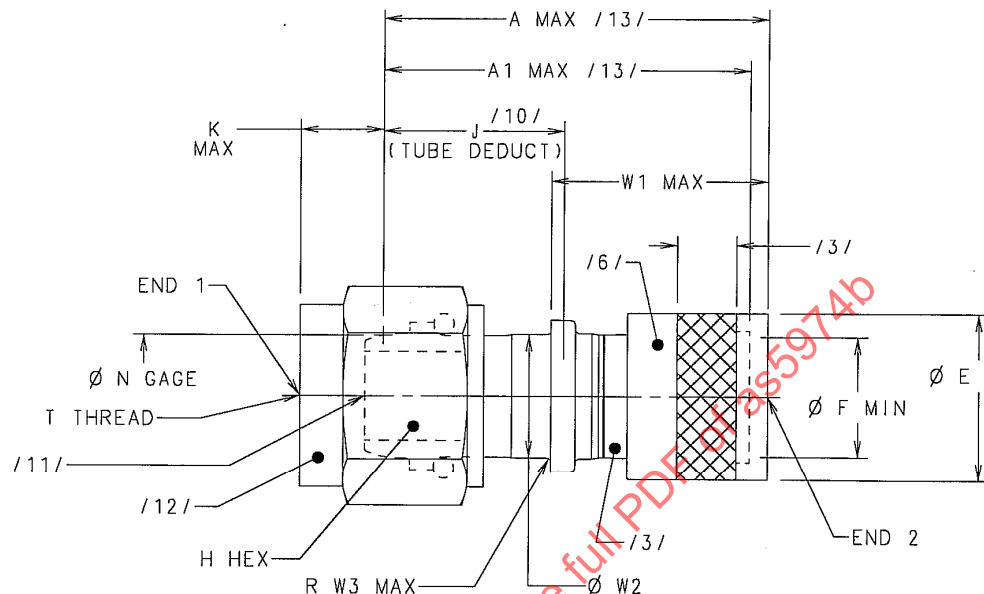
FIGURE 1 - ADAPTER, SWAGE
