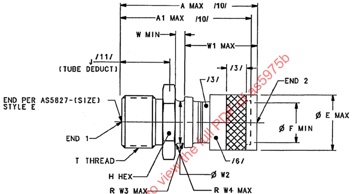
FIGURE 1 - ADAPTER, SWAGE
