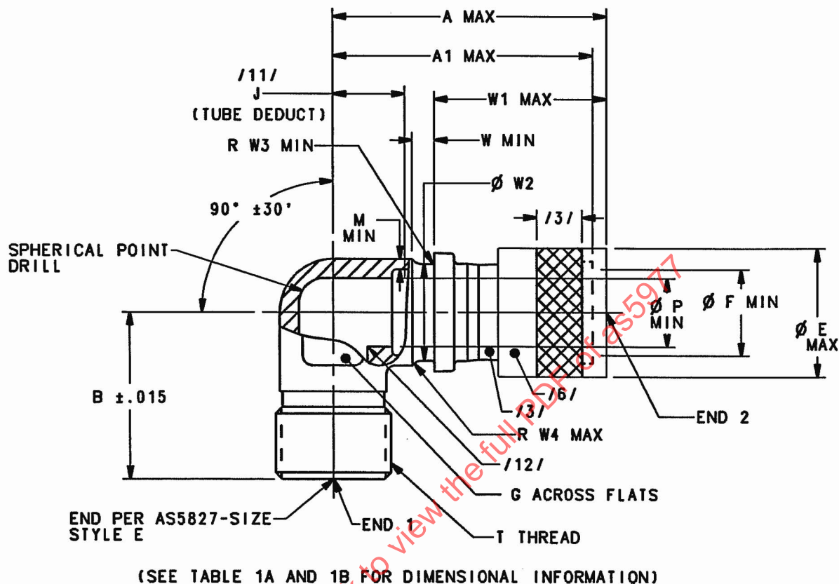
FIGURE 1 - ELBOW, 90°, SWAGE
