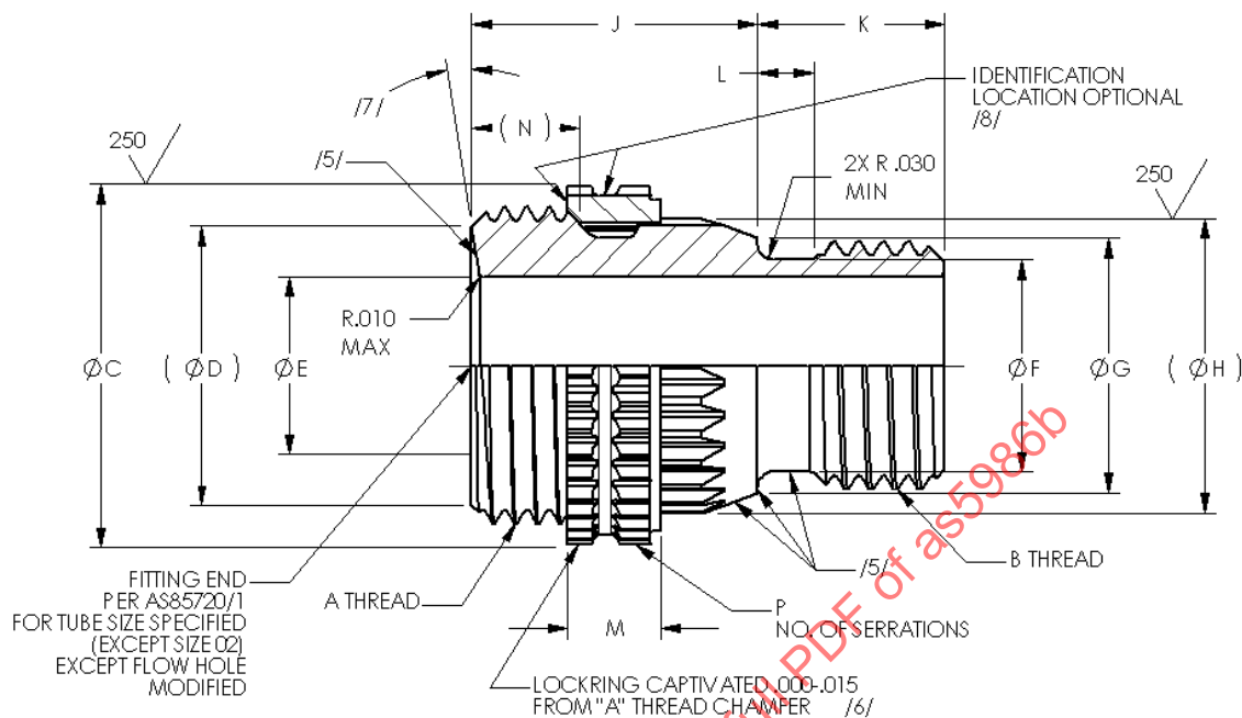
FIGURE 1 – ADAPTER, ASSEMBLY
