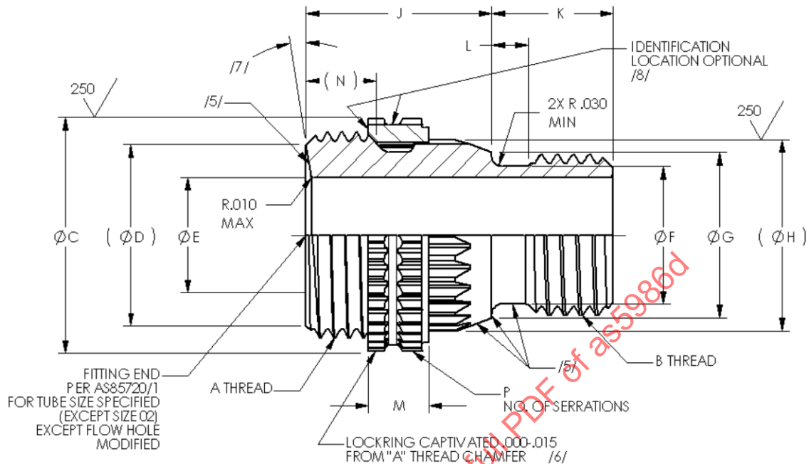
FIGURE 1 - ADAPTER, ASSEMBLY
