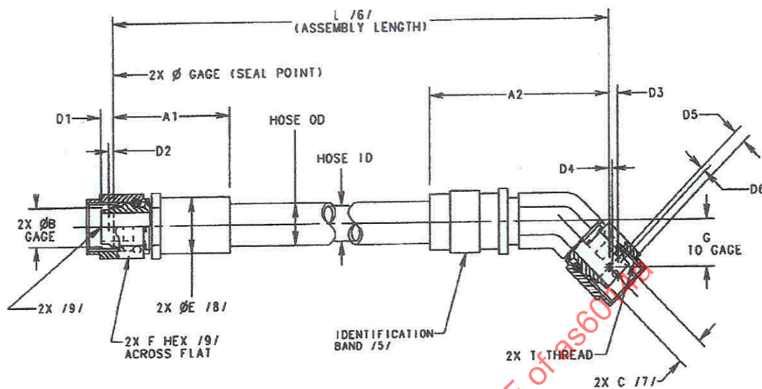
FIGURE 1 - FLARELESS HOSE ASSEMBLY, STRAIGHT TO 45 DEGREE ELBOW
