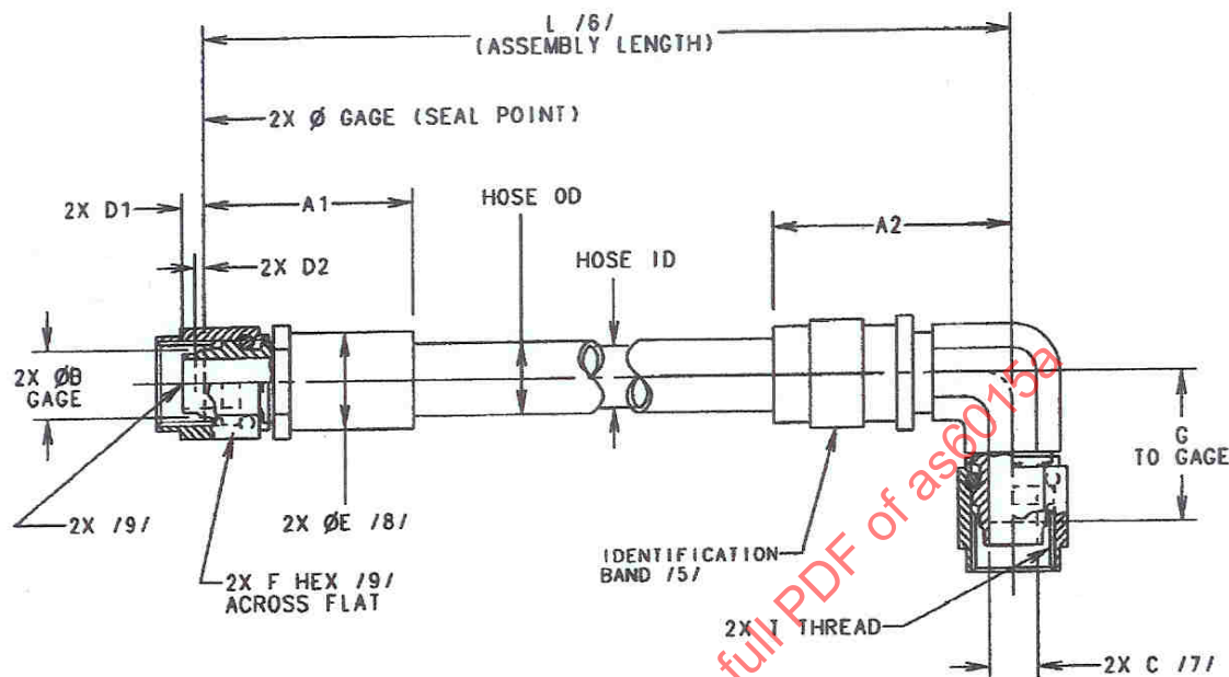
FIGURE 1 - FLARELESS HOSE ASSEMBLY, STRAIGHT TO 90 DEGREE ELBOW
