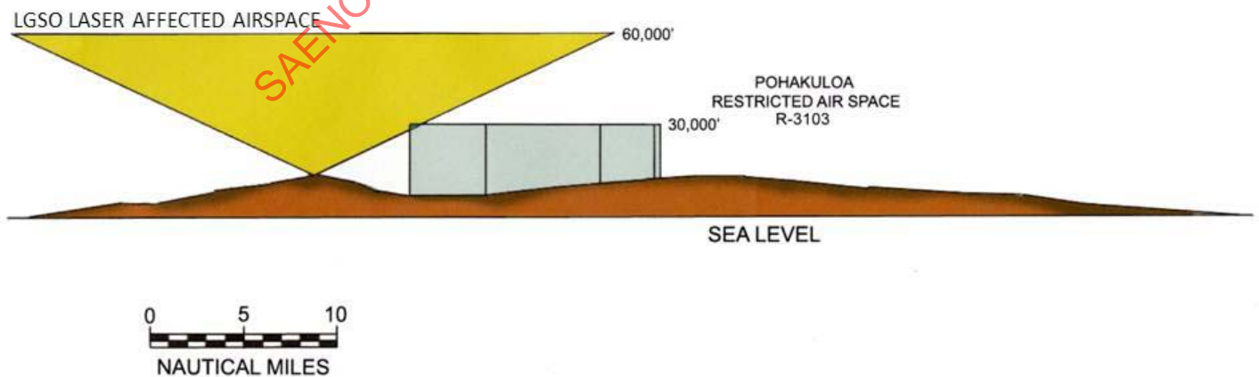
FIGURE C5 - ELEVATION VIEW OF THE BIG ISLAND, SHOWING THE LGSO LASER-AFFECTED AIRSPACE AND RESTRICTED AIRSPACE R-3103
