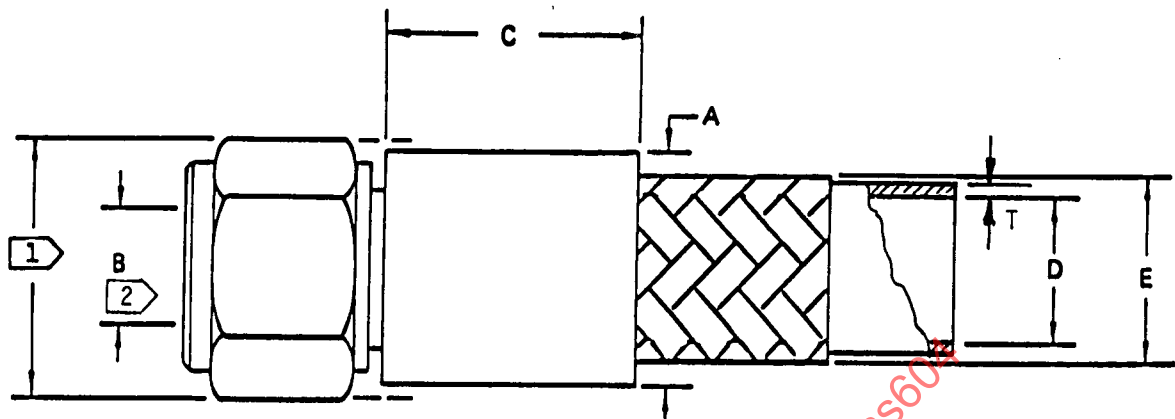
HOSE AND FITTING DIMENSIONS
