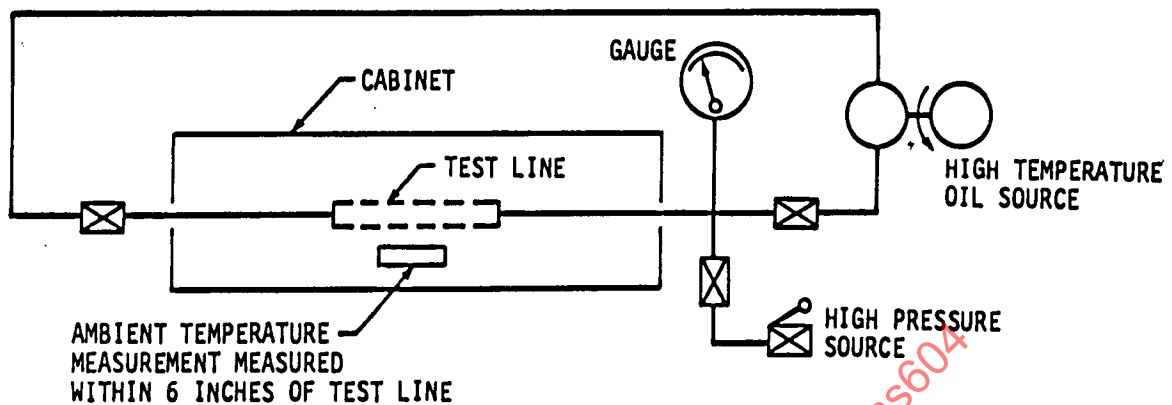
TYPICAL SETUP FOR THERMAL SHOCK TESTING
