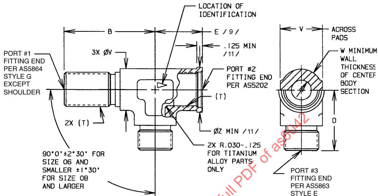
FIGURE 1 - FITTING, TEE, BULKHEAD END, PORT #2 SHOWN AS NON-REDUCER
