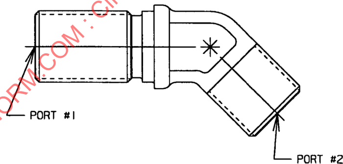
FIGURE 2 - FITTING, ELBOW, 45°, BULKHEAD END, NON-REDUCER SHOWN, SAME AS FIGURE 1 EXCEPT AS SHOWN
