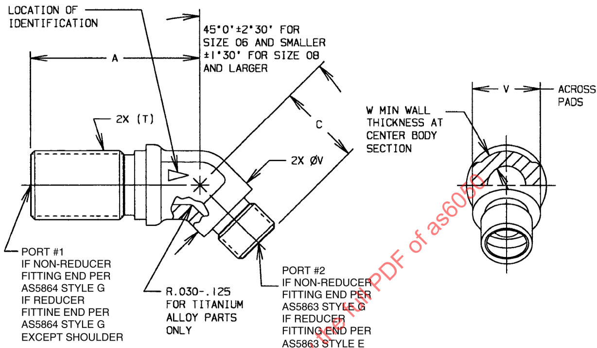
FIGURE 1 - FITTING, ELBOW, 45°, BULKHEAD END, PORT #1 SHOWN AS NON-REDUCER, PORT #2 SHOWN AS REDUCER
